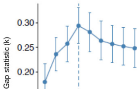
Gap statistic
