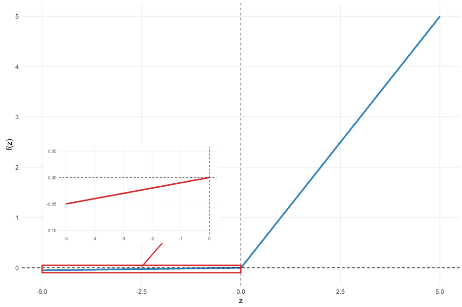
Leaky ReLU
