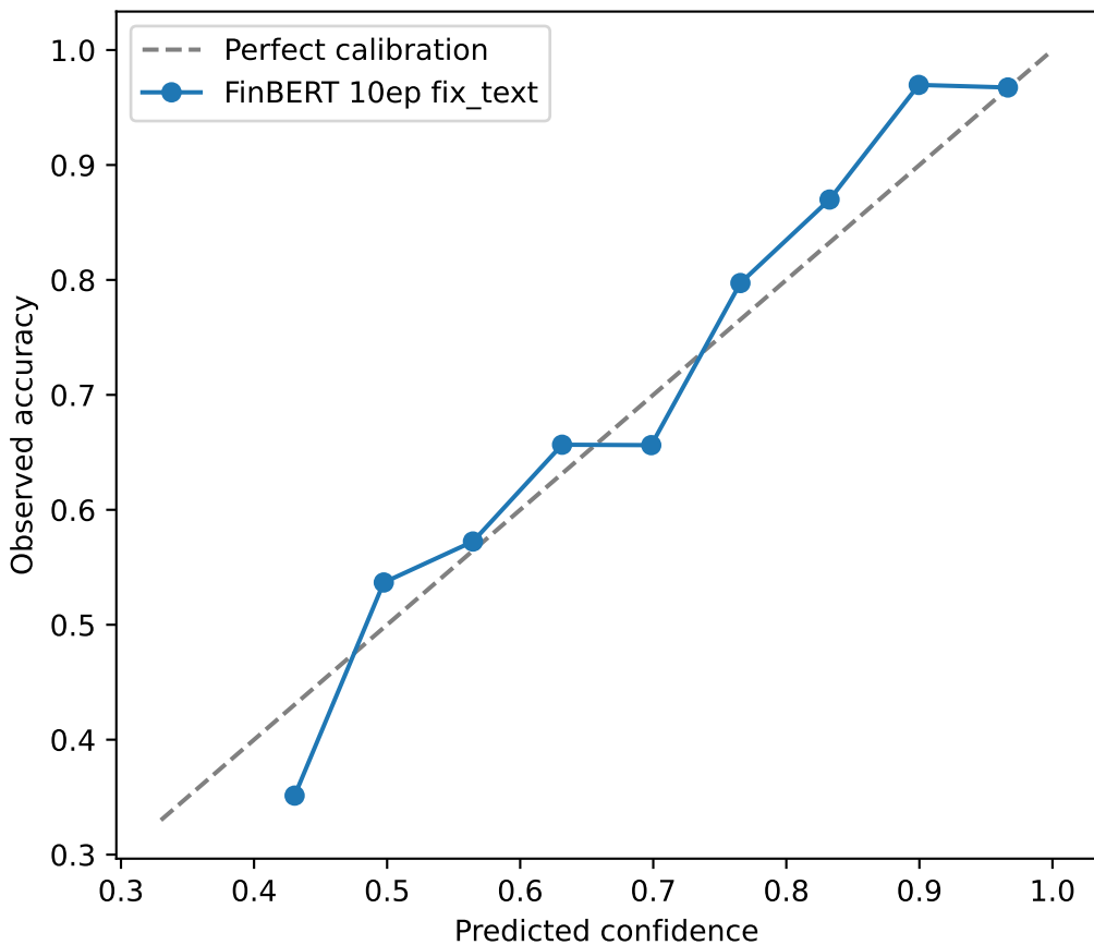
Calibration curve (OOF, 10-fold)
