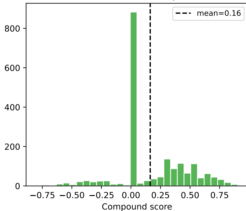
Bullish - VADER compound
