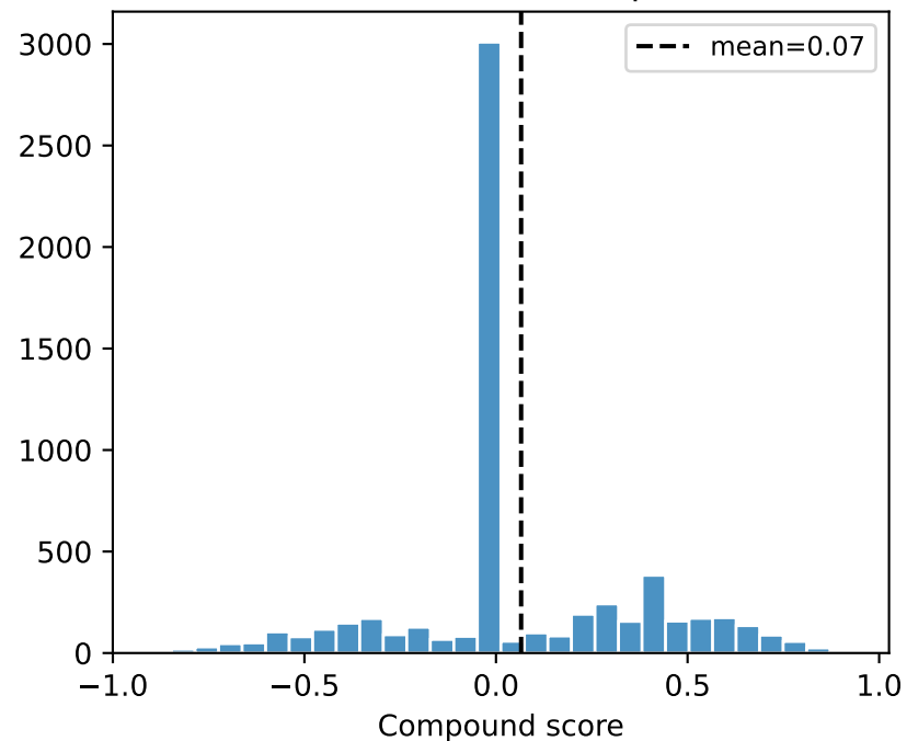
Neutral - VADER compound
