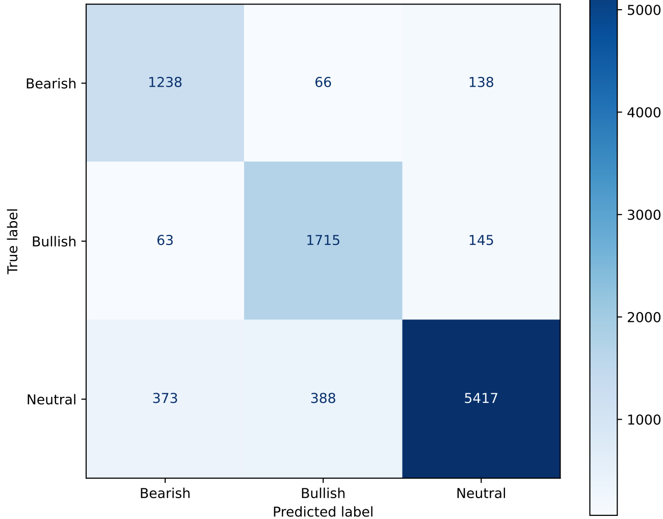
Final model — Stacking-6 (LR meta) | +fine-tuned — Absolute
