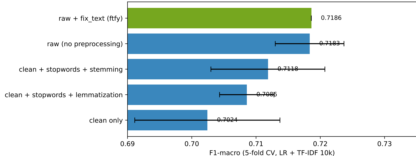
Preprocessing Ablation Study (green = best)
