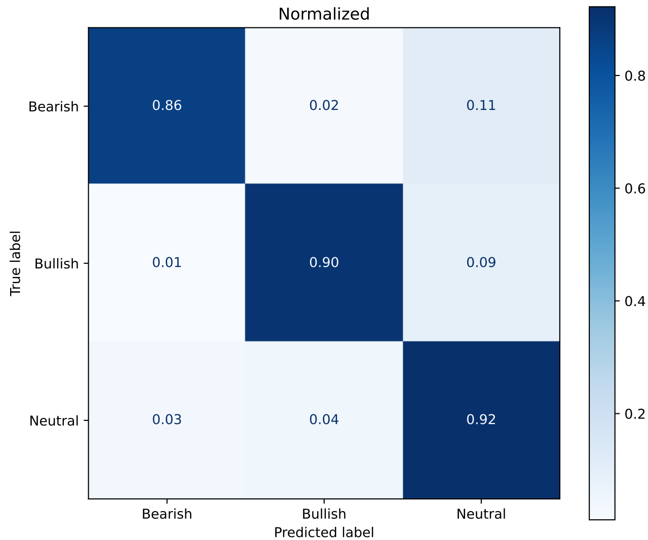
Twitter-RoBERTa-large-topic-sentiment-latest fine-tuned
