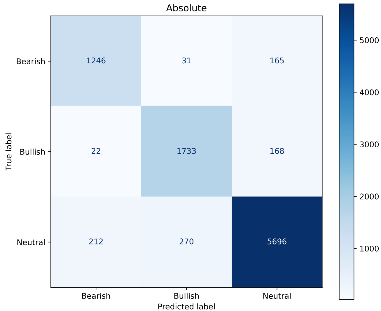
Twitter-RoBERTa-large-topic-sentiment-latest fine-tuned
