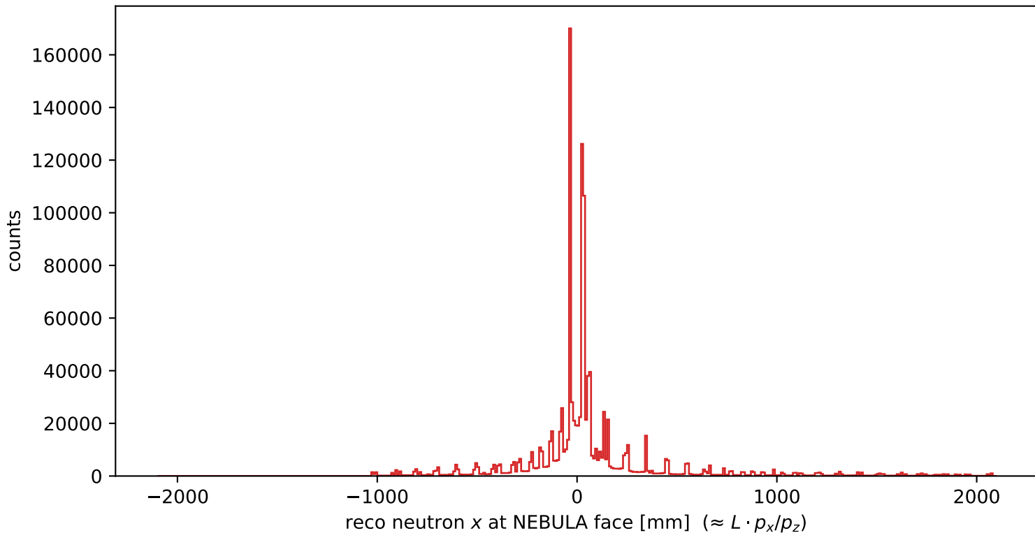
Fig A3: NEBULA reco-x discrete bands (60-bar \times \sim 122 mm pitch)
