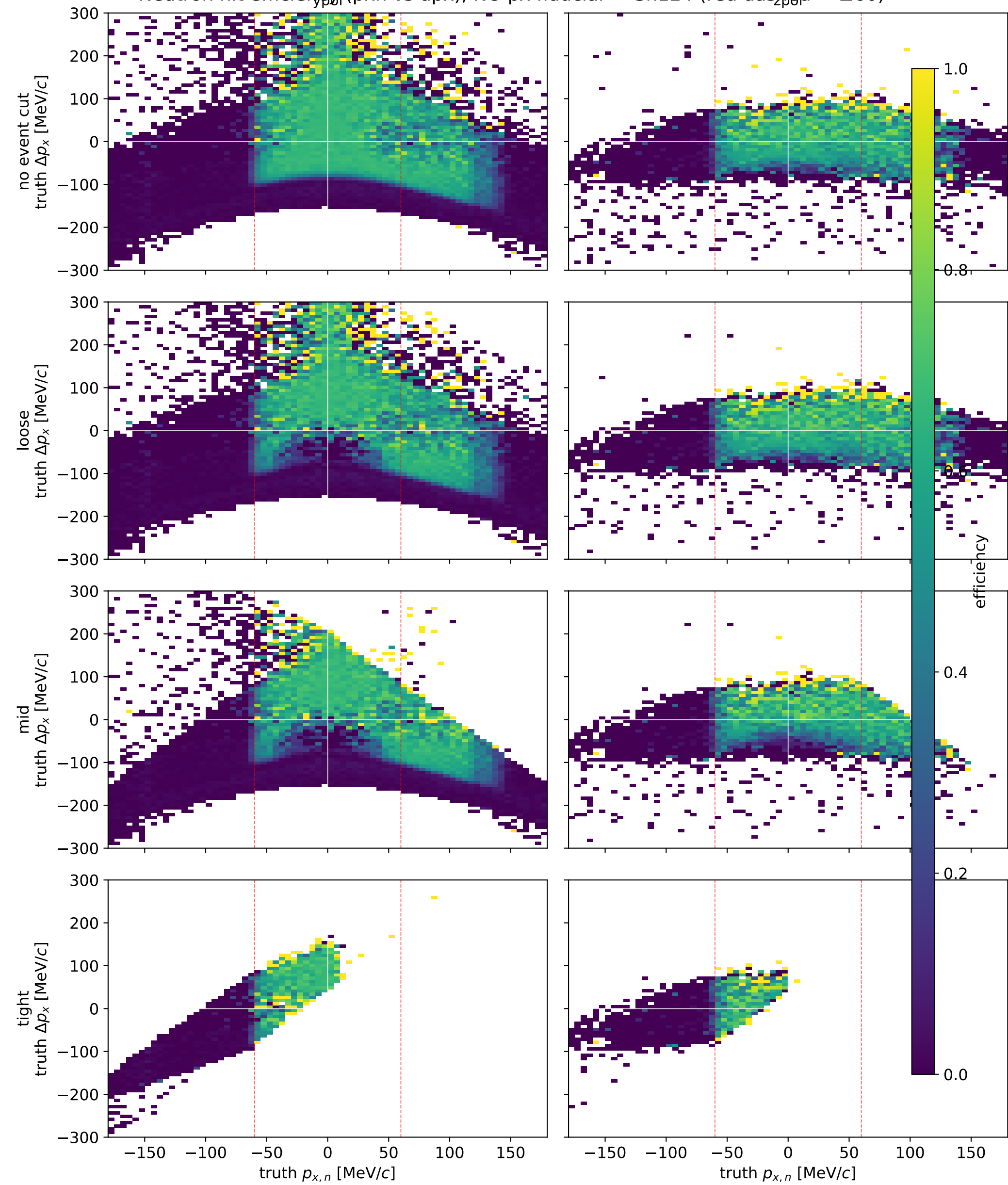
Neutron hit efficiency, (pxn vs dpx), NO px fiducial — Sn124 (red dashed = \pm 60 )
