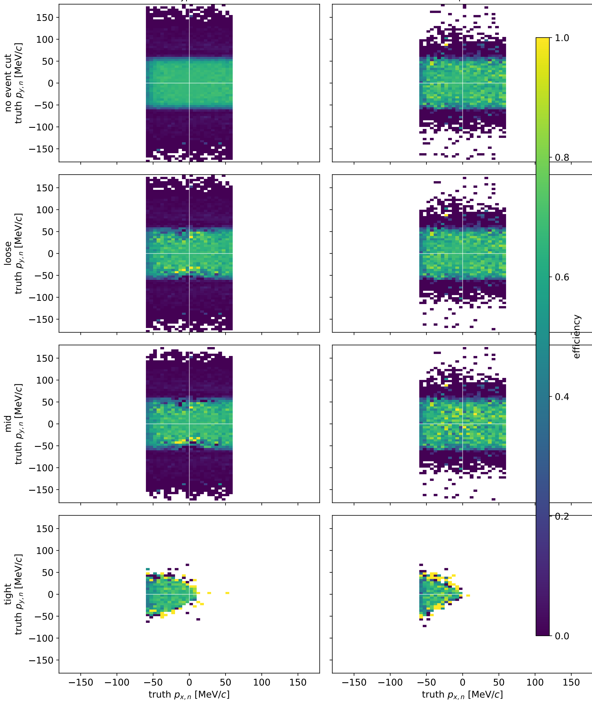
Neutron hit efficiency (pxn vs pyn) by event-quality cut — Sn124, px60 fiducial
