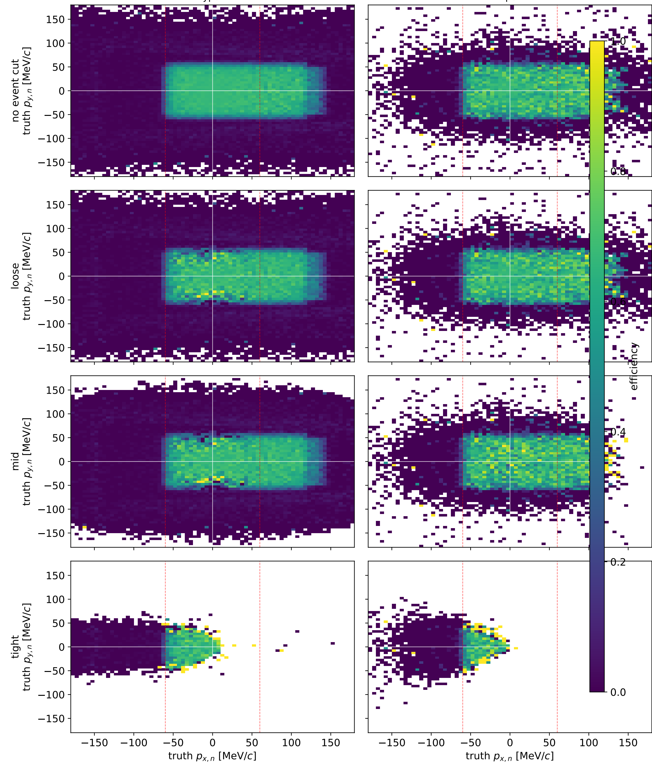
Neutron hit efficiency 1 (pxn vs pyn), NO px fiducial — Sn124 (red dashed = \pm 60 )
