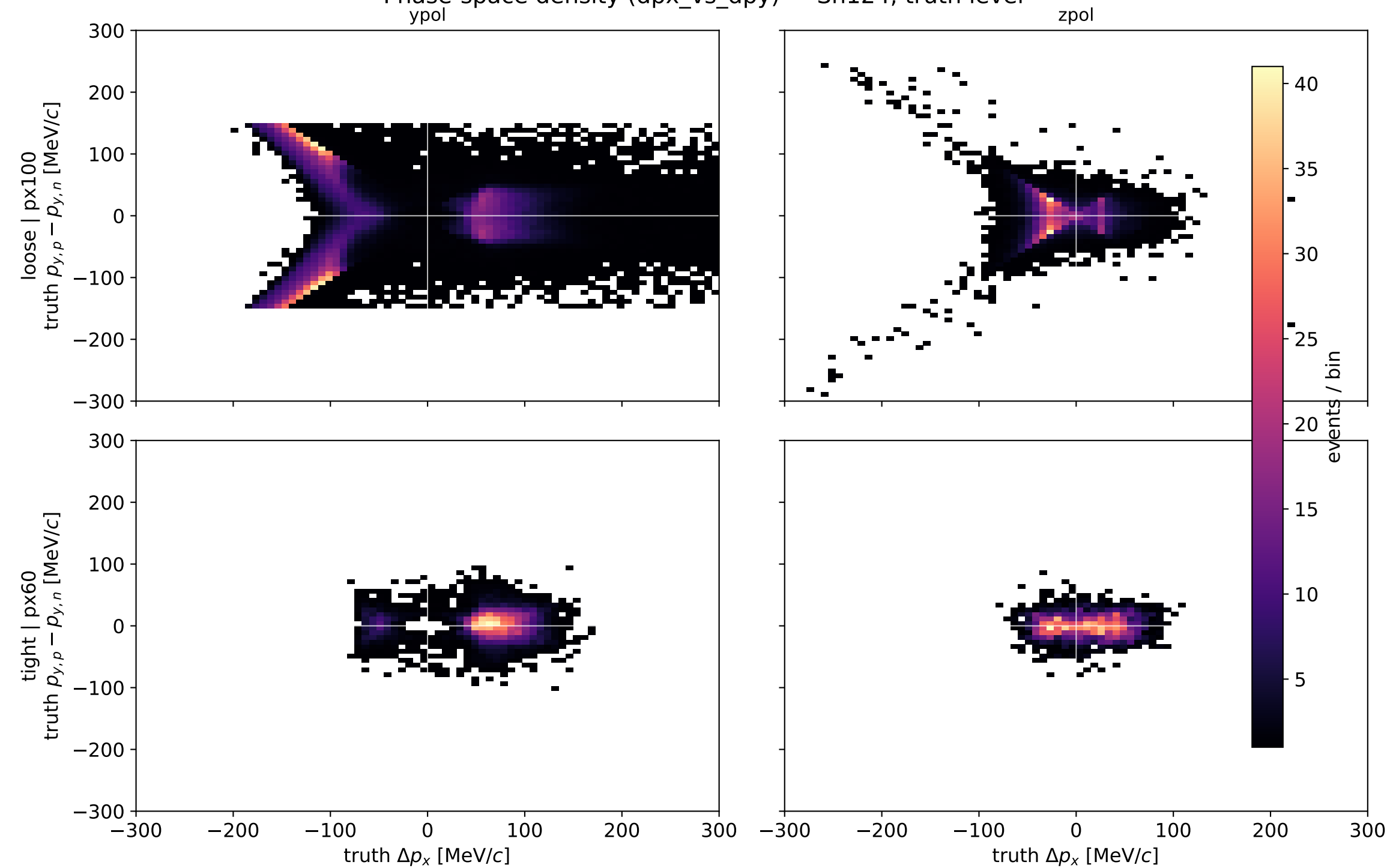
Phase-space density (dpx_vs_dpy) — Sn124, truth level
