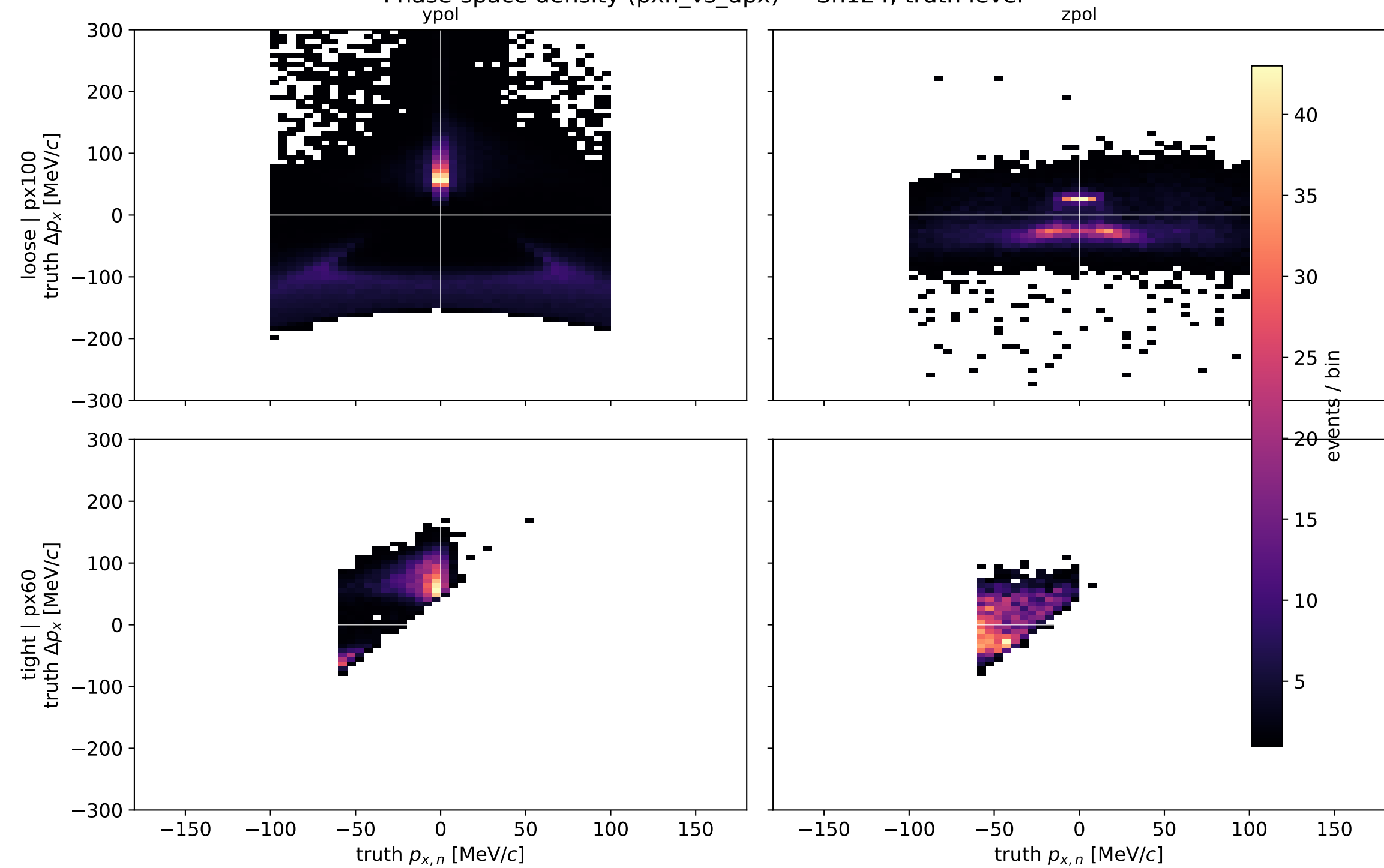
Phase-space density (pxn_vs_dpx) — Sn124, truth level
