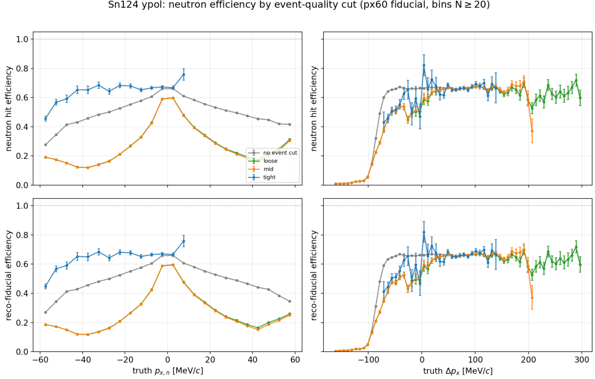
Figure 22: y-pol neutron efficiency versus event-quality cut (px60 truth fiducial). Four curves = none (no event cut) / loose / mid / tight. Top row = neutron hit efficiency, bottom row = reco-fiducial efficiency; left column vs truth p_{x,n} , right column vs truth \Delta p_x . Efficiency is \epsilon(x) = N_{\text{hit}}(x\text{-bin})/N_{\text{fid}}(x\text{-bin}) ; only bins with N_{\text{fid}} \geq 20 are drawn.
