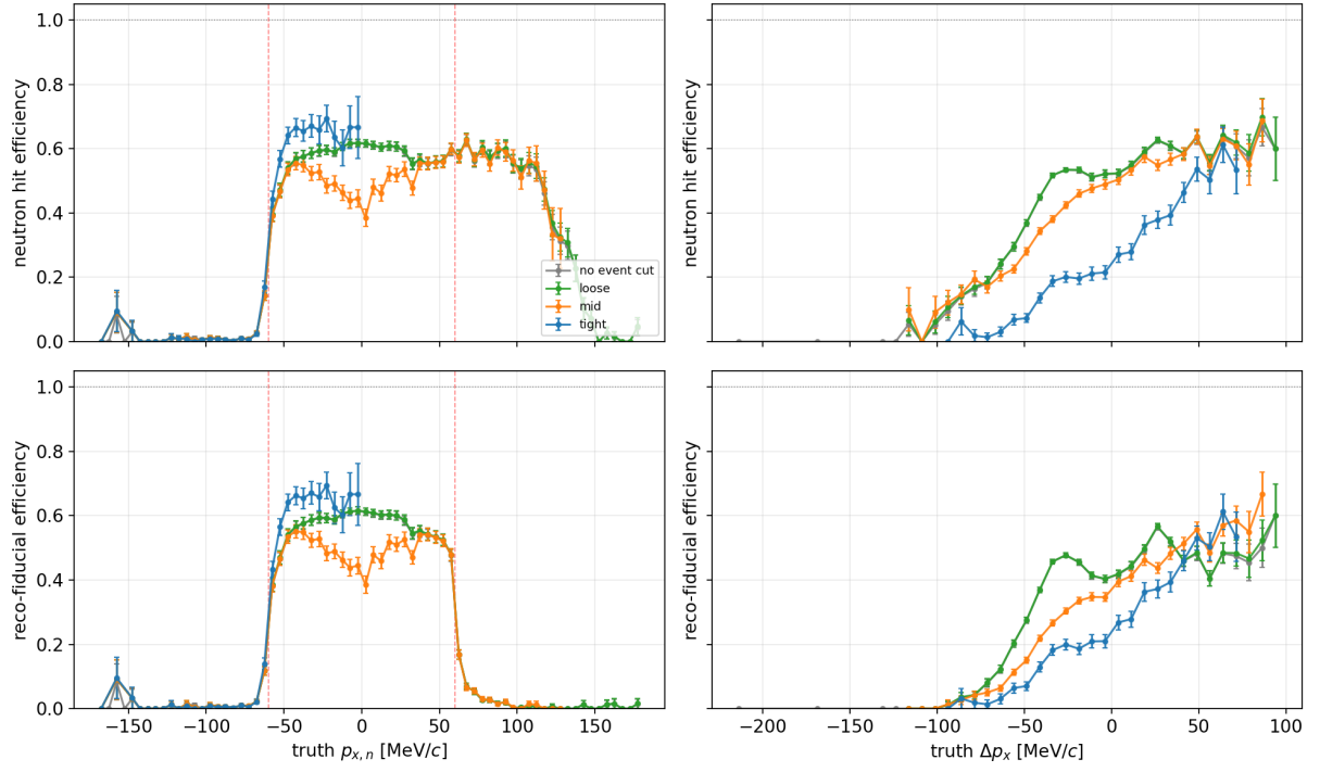
Figure 26: z-pol: the corresponding full-range efficiency curves.
