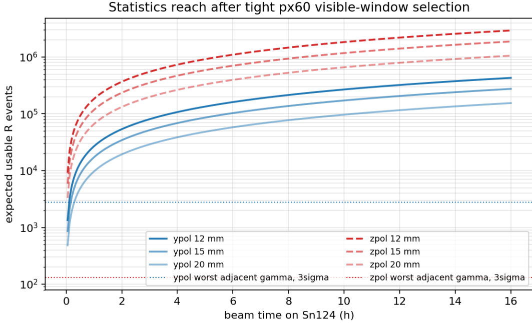
Figure 29: Usable R -event reach after the tight px60 visible-window selection for the Sn124 inventory target options.
