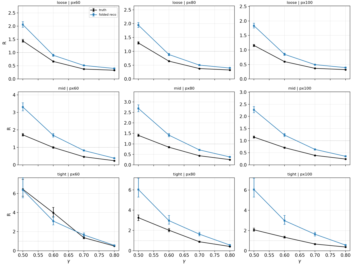
Figure 16: z-pol: the same 9-combination grid.
