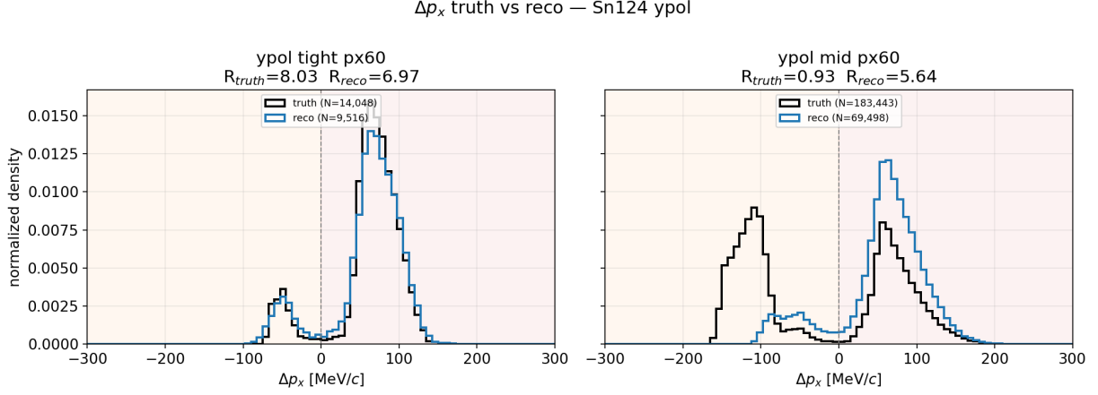
Figure 17: y-pol normalized \Delta p_x histograms. Black = truth (truth event plane + truth momenta), blue = reco (reco event plane + NN proton + reconstructed neutron). Red shading = \Delta p_x > 0 ( R numerator), orange = \Delta p_x < 0 ( R denominator). Tight px60 and mid px60 side by side.
