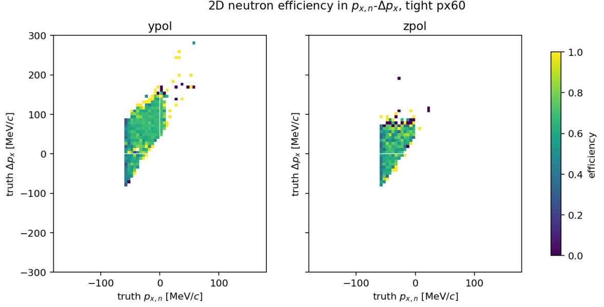
Figure 8: Two-dimensional neutron efficiency in truth p_{x,n} versus truth \Delta p_x . This is the most direct efficiency map for the sign observable because it links neutron acceptance to the final numerator/denominator of R .
