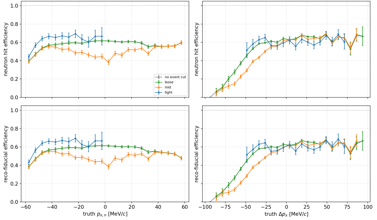
Figure 23: z-pol: the corresponding efficiency curves. The z-pol “none” curve has limited statistics in some bins.
