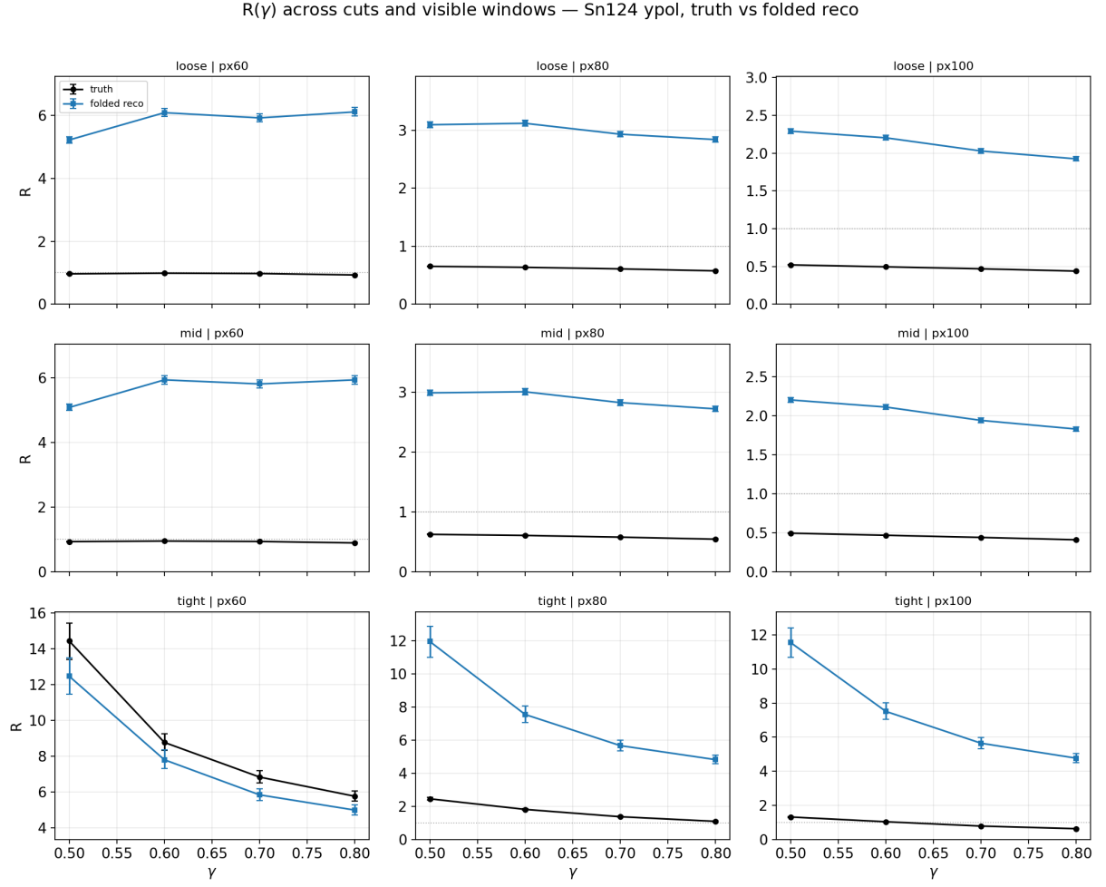
Figure 15: y -pol R(\gamma) across the 9 cut combinations (rows = loose/mid/tight, columns = px60/px80/px100), Sn124. Black = truth-level R , blue = folded reco R , error bars from bootstrap.
