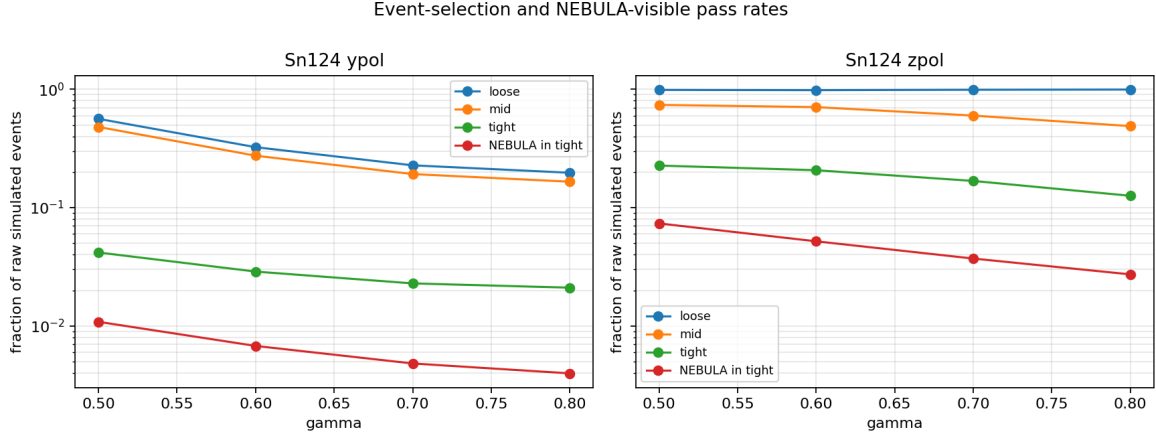
Figure 4: Sn124 selection pass rates versus \gamma . The final NEBULA-visible tight sample is the small fraction that can enter the folded R observable.
