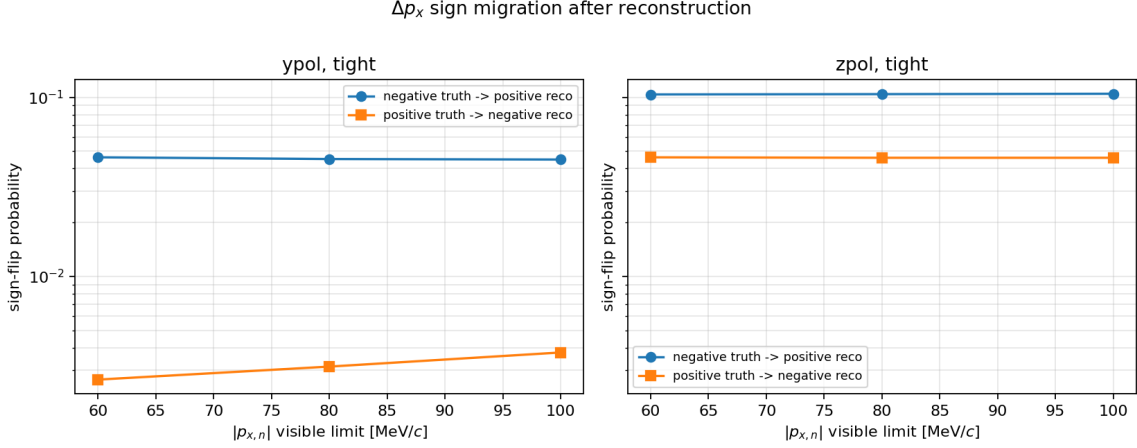
Figure 14: \Delta p_x sign-flip probability versus neutron visible-window size for tight selections. Sign migration is defined as the conditional probability P(\text{reco sign} | \text{truth sign}) with truth sign = \text{sgn}(\Delta p_x^{\text{truth}}) and reco sign = \text{sgn}(\Delta p_x^{\text{reco}}) ; the diagonal (truth \rightarrow same sign) is the retention rate and the off-diagonal (truth \rightarrow opposite sign) is the flip rate.
