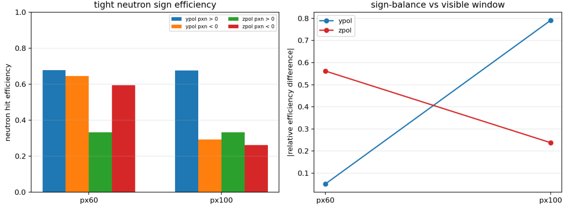
Figure 10: Neutron sign efficiency balance for tight selections. The y-pol sample gives the stable sign-balance comparison; z-pol tight has very small positive- p_{x,n} statistics in this diagnostic.
