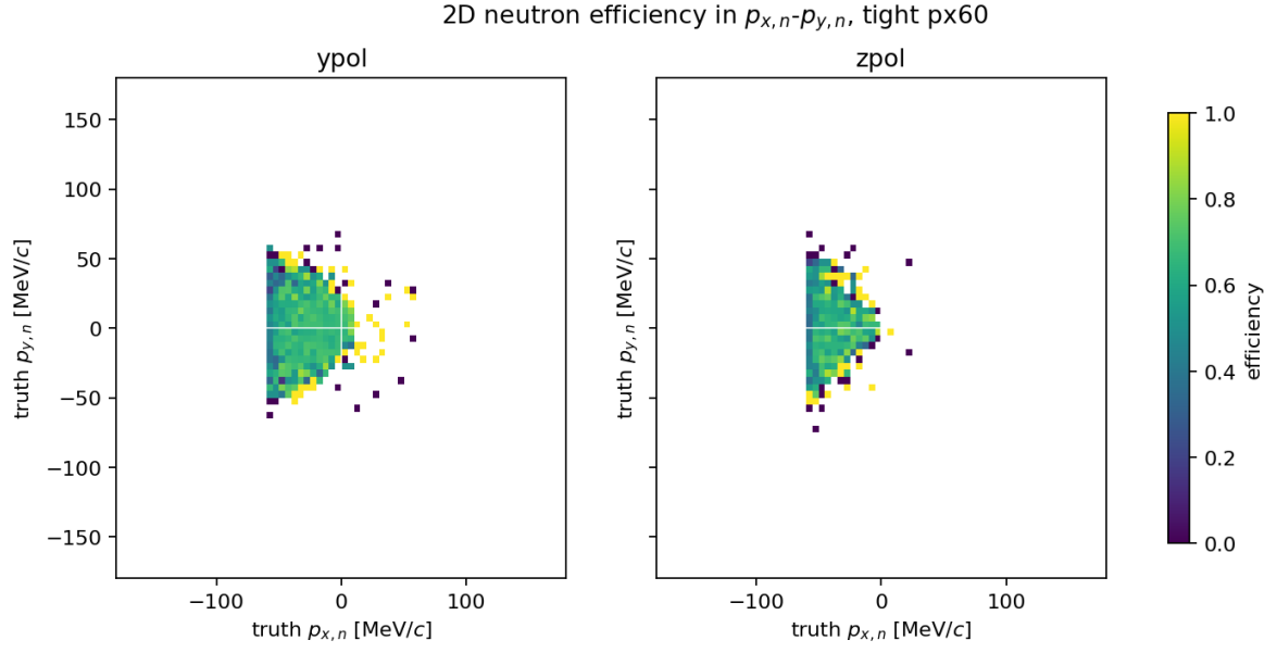
Figure 6: Two-dimensional neutron efficiency in truth p_{x,n} versus truth p_{y,n} for tight px60. Empty white regions are outside the populated/usable diagnostic phase space.
