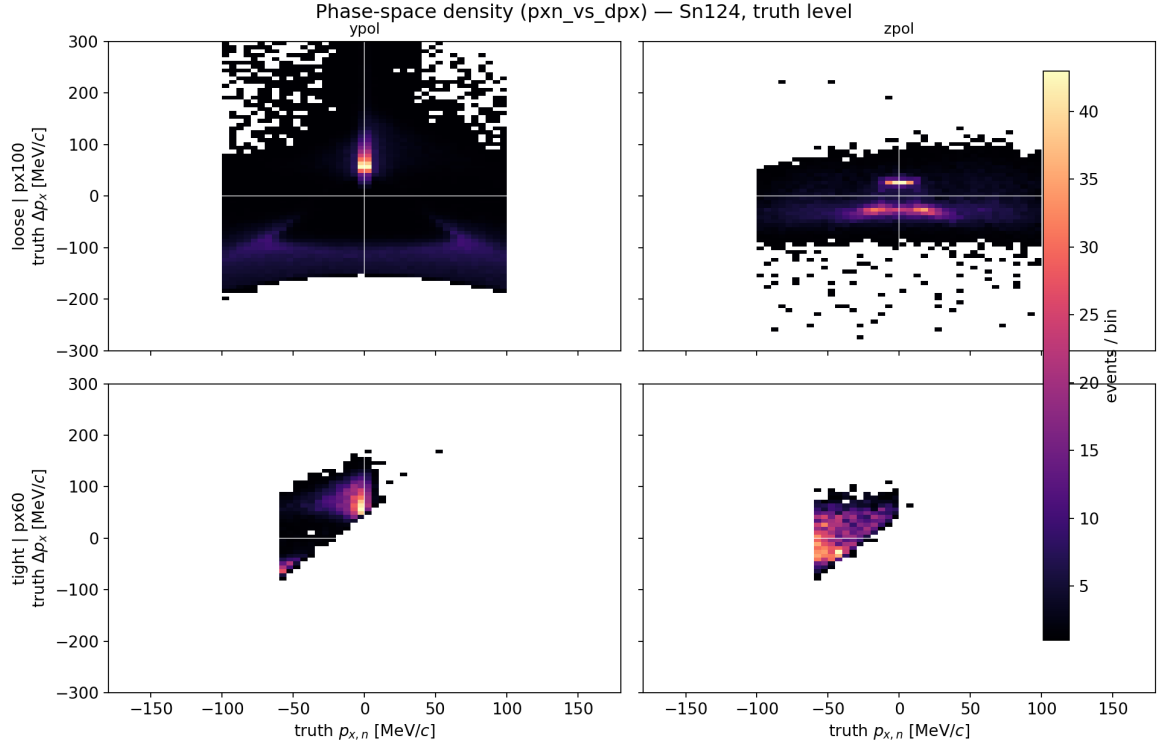
Figure 19: Truth-level phase-space density (event counts per bin, not efficiency). Top row = loose px100, bottom row = tight px60, columns = y-pol/z-pol. It answers “which region of truth phase space does this cut keep?”.
