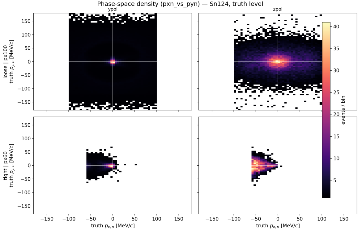
Figure 20: Same, truth p_{x,n} vs p_{y,n} neutron transverse plane.
