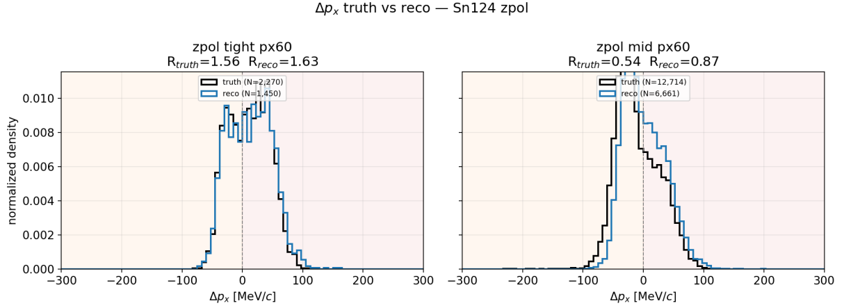
Figure 18: z-pol: the corresponding \Delta p_x truth vs reco overlay.
