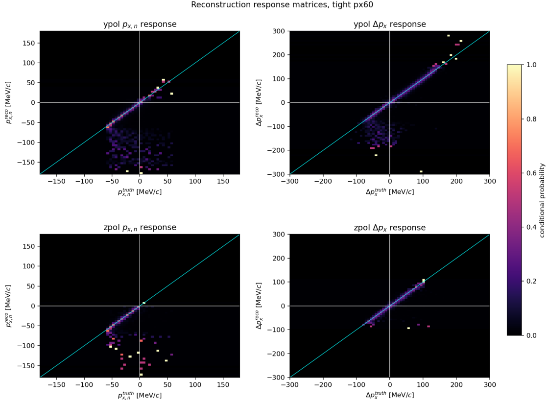
Figure 11: Conditional response matrices for reconstructed p_{x,n} and reconstructed \Delta p_x in tight px60. The cyan line is the diagonal. Black regions are bins without usable diagnostic statistics.
