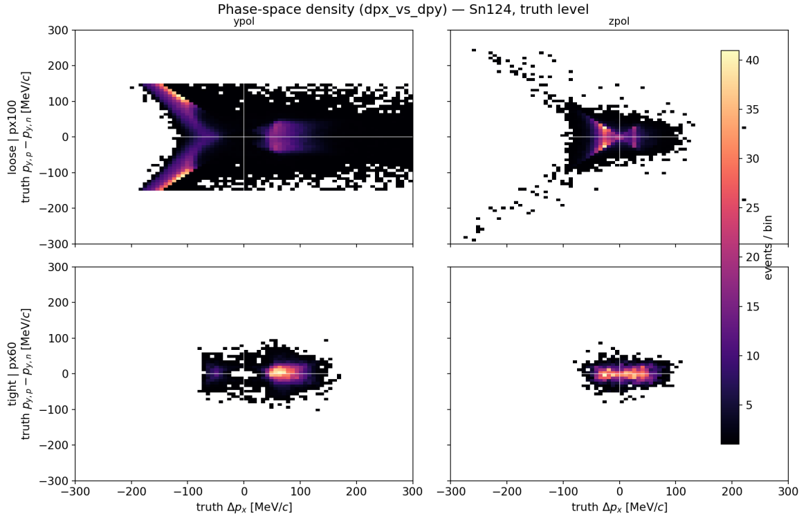
Figure 21: Same, truth \Delta p_x vs (p_{y,p} - p_{y,n}) momentum-asymmetry plane. The tight cut compresses events toward the reaction plane.
