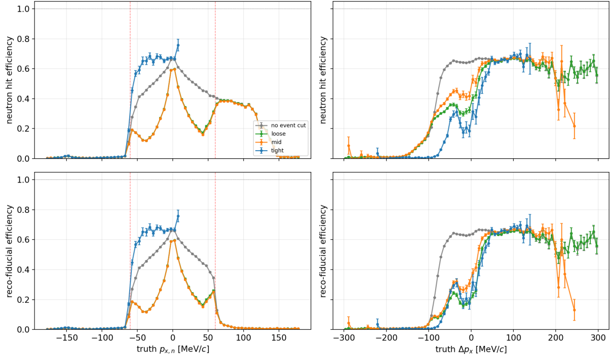
Figure 25: y-pol neutron efficiency across the full p_{x,n} range, no px fiducial. Red dashed = \pm 60 MeV/c (the px60 window boundary). Top row = neutron hit efficiency, bottom row = reco-fiducial efficiency. Four curves as before (none/loose/mid/tight).
