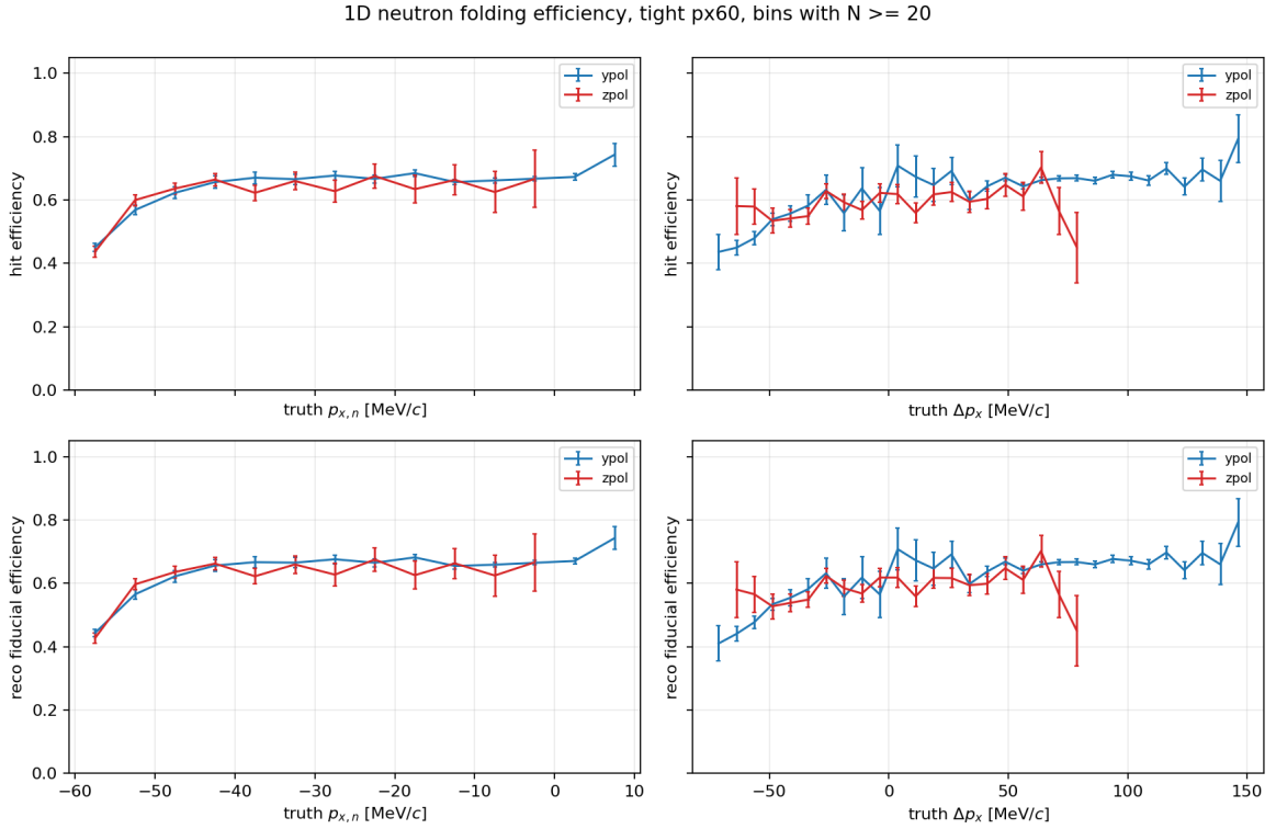
Figure 9: One-dimensional neutron hit and reconstructed-fiducial efficiencies for bins with at least 20 truth events. In the populated core, the efficiency is typically around 0.55–0.70 rather than flat at unity.
