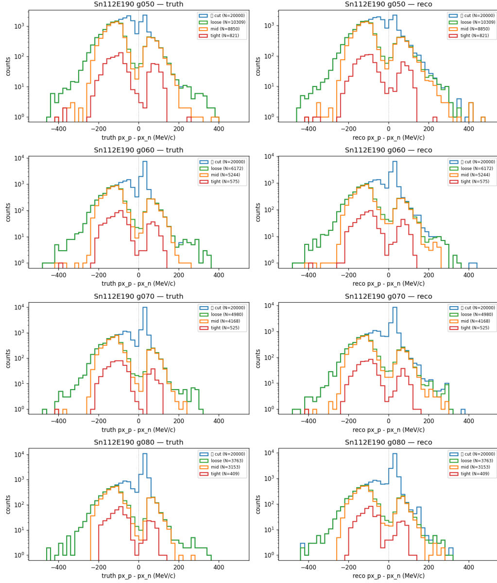
图 10: \Delta p_x^{\text{rot}} 在四 cut 下的叠加 (Sn112E190)。4 行 = 4 gammas, 列 = truth (A) / reco mixed (B). 蓝 = 无 cut, 绿 = loose, 橙 = mid, 红 = tight.
