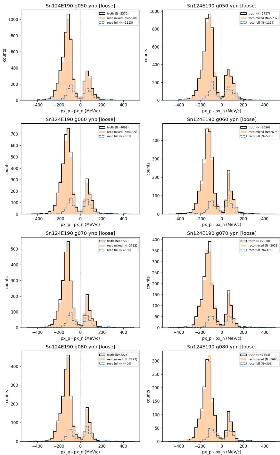
图 5: \Delta p_x^{\text{rot}} 分布 (Sn124E190, loose cut)。黑 step = A truth, 橙填充 = B reco mixed, 蓝虚线 = C full reco.
