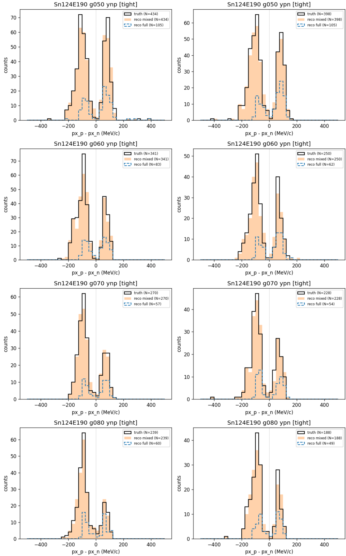
图 9: \Delta p_x^{\text{rot}} 分布 (Sn124E190, tight cut)。黑 step = A truth, 橙填充 = B reco mixed, 蓝虚线 = C full reco.
