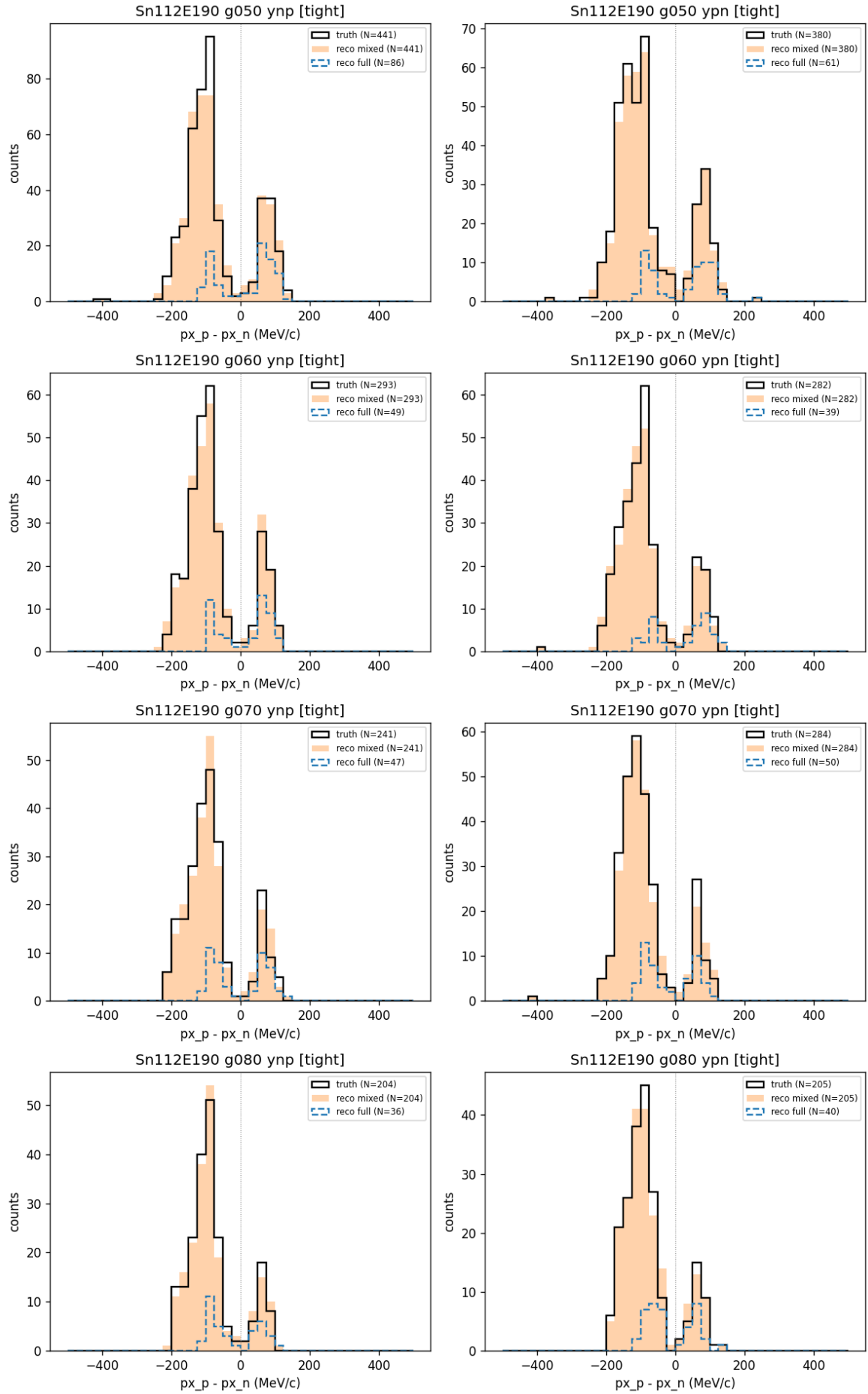
图 8: \Delta p_x^{\text{rot}} 分布 (Sn112E190, tight cut)。黑 step = A truth, 橙填充 = B reco mixed, 蓝虚线 = C full reco.
