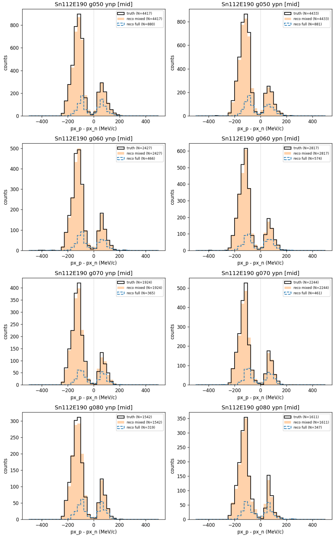
图 6: \Delta p_x^{\text{rot}} 分布 (Sn112E190, mid cut)。黑 step = A truth, 橙填充 = B reco mixed, 蓝虚线 = C full reco.
