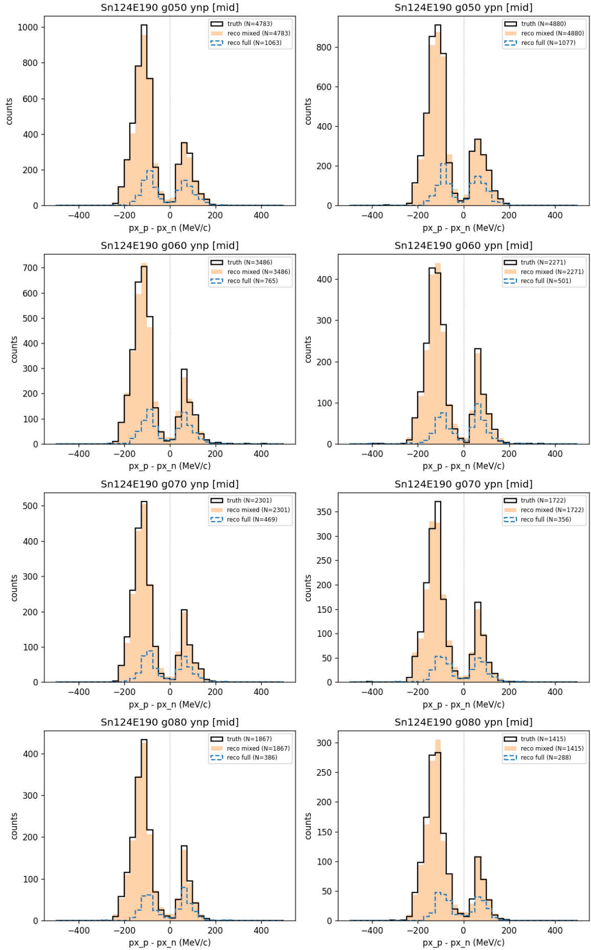
图 7: \Delta p_x^{\text{rot}} 分布 (Sn124E190, mid cut)。黑 solid = A truth, 橙填充 = B reco mixed, 蓝虚线 = C full reco.
