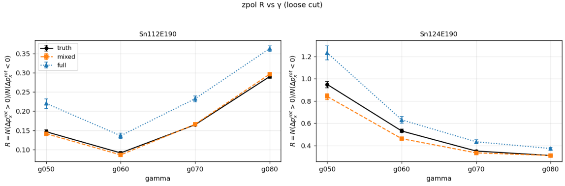
图 8: zpol R_x^{\text{rot}} vs gamma (loose cut).
