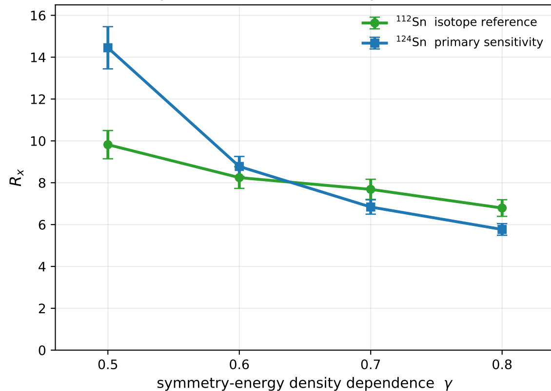
The detector changes the scale, not the physical ordering Ideal model prediction (generator level, before any detector)
