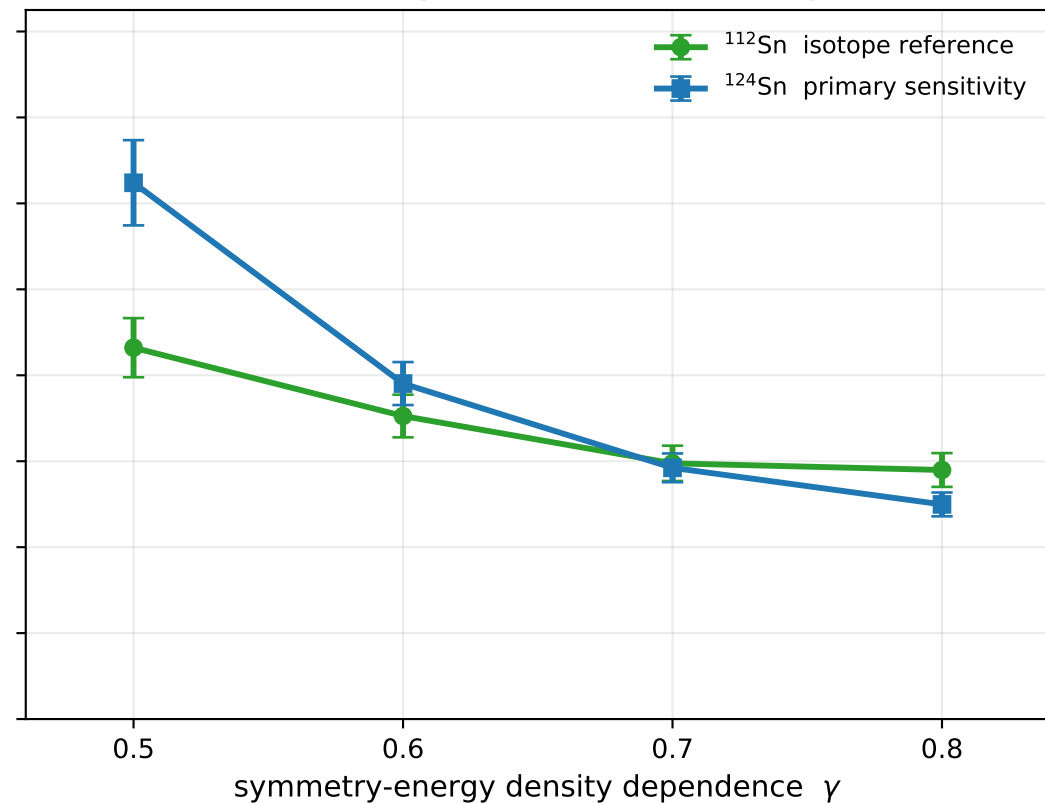
After detector + reconstruction (reconstructed proton, neutron, event plane)
