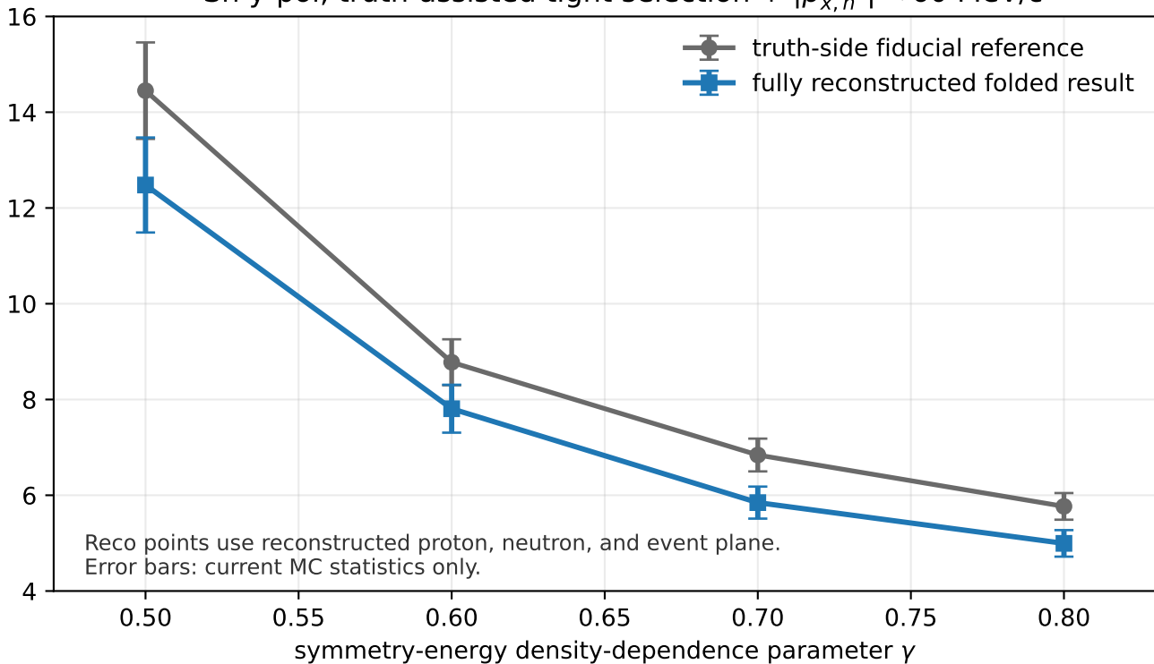
^{124}\text{Sn} y-pol, truth-assisted tight selection + |p_{x,n}^{\text{reco}}| < 60 \text{ MeV}/c
