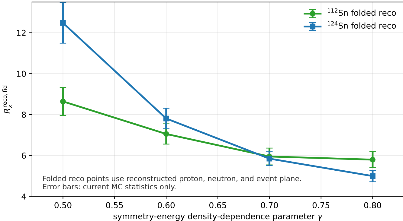
y-pol isotope comparison, truth-assisted tight selection + |p_{x,n}^{\text{reco}}| < 60 \text{ MeV}/c
