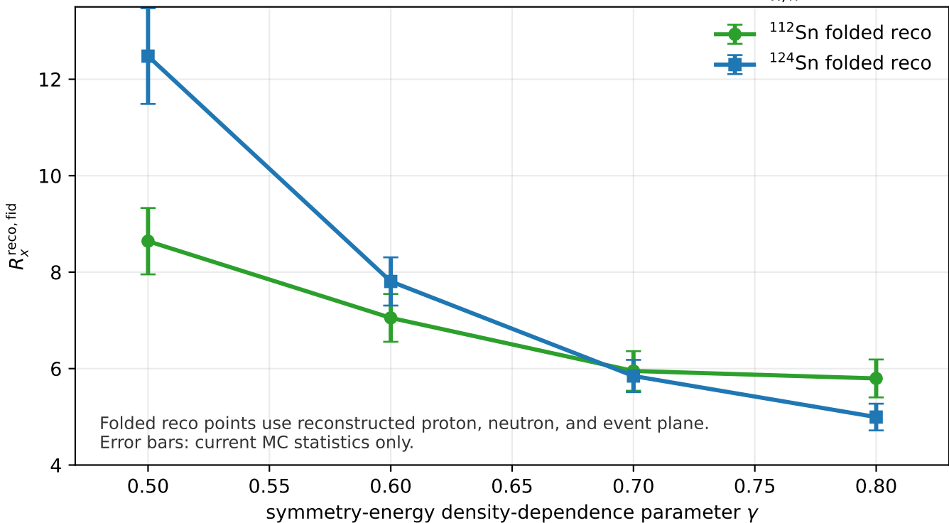
y-pol isotope comparison: truth-defined tight quality class; |p_{x,n}^{\text{reco}}| < 60 MeV/c
