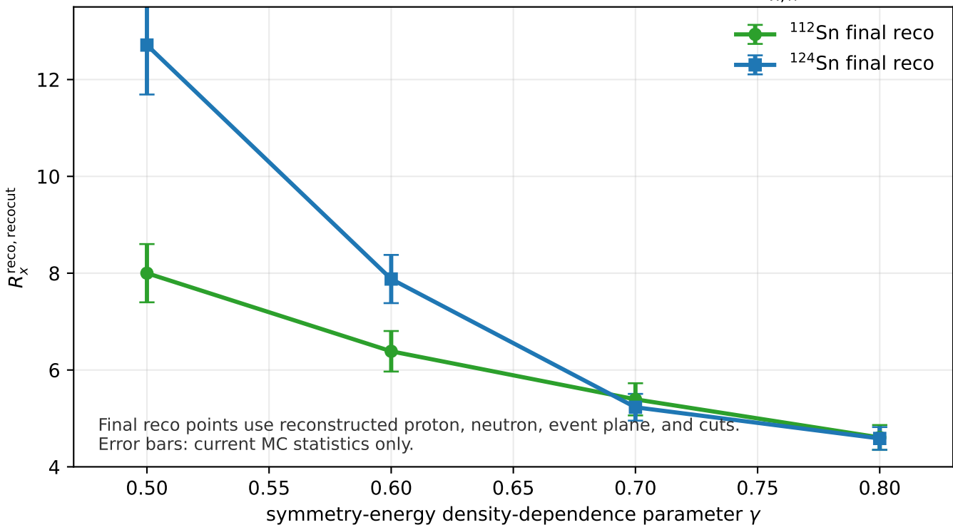
y-pol isotope comparison: reco-defined tight quality class; |p_{x,n}^{\text{reco}}| < 60 \text{ MeV}/c
