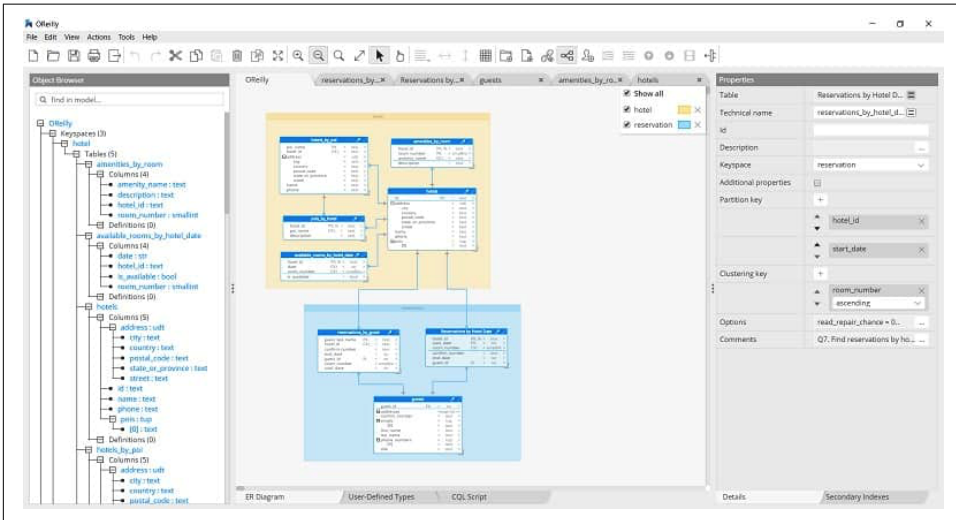
Figure 5-11. An entity-relationship diagram for hotel and reservation data in Hacklade
