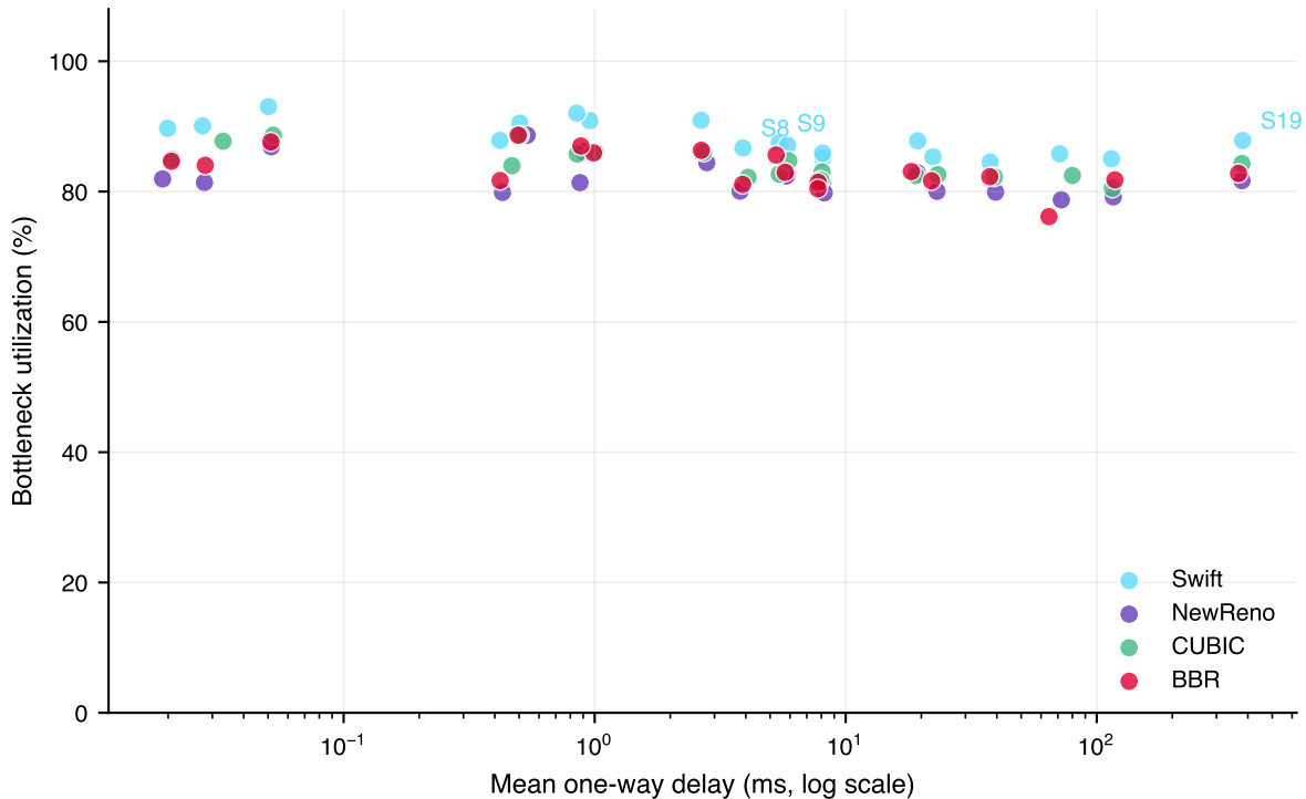
Utilization-delay trade-off (TCP-only, 19 scenarios)
