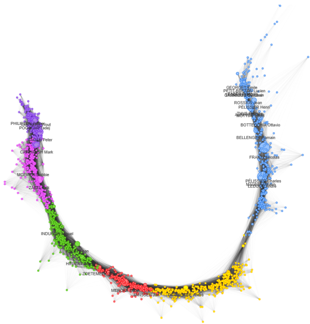
Fig. 5. Points Network
