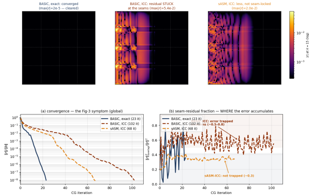
Fig. 13 — Exact vs inexact at the seams: Fig 3 (panel a) shows only the convergence gap; the fields + seam fraction (b) show WHERE the inexact error accumulates residual field at the same iteration k=15 (white dotted = subdomain seams)
