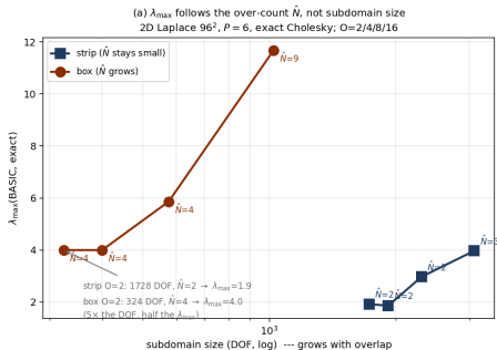
Fig. 11 — Controls: (a) the over-count \hat{N} (not size) sets \lambda_{\max} ; (b) a coarse space and sASM fix opposite ends of the spectrum --- you need both
