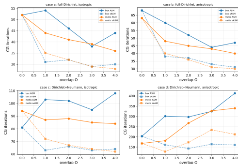
3D unstructured P1 FEM: ASM vs sASM (CG iterations)
