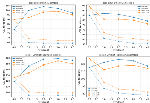
2D unstructured P1 FEM: ASM vs sASM (CG iterations)
