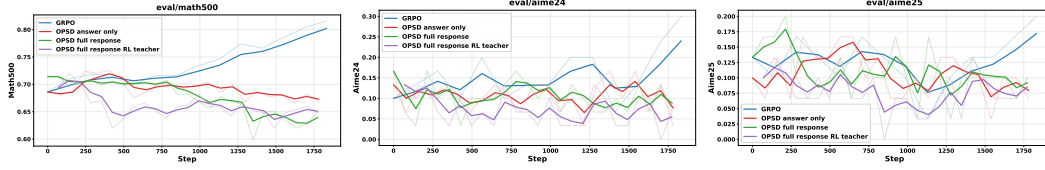
Figure 3: Qwen3-1.7B, trained on OpenThoughts. OPSD fails to improve student.
