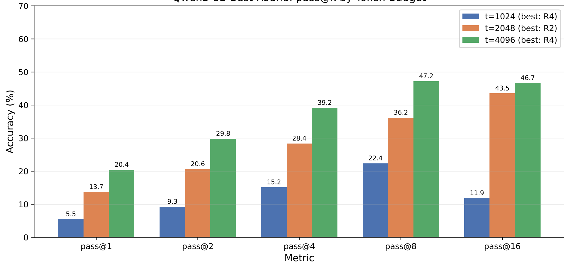
Qwen3-8B Best Round: pass@k by Token Budget
