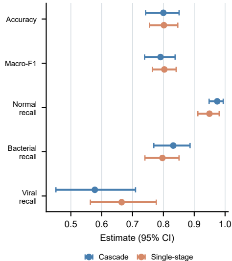
c Cascade versus single-stage
