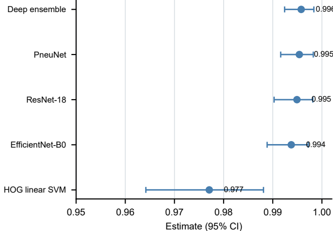
c Conditional Stage 2 ROC-AUC (n = 417; 266 groups)
