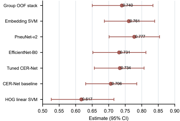
d Conditional Stage 2 PR-AUC
