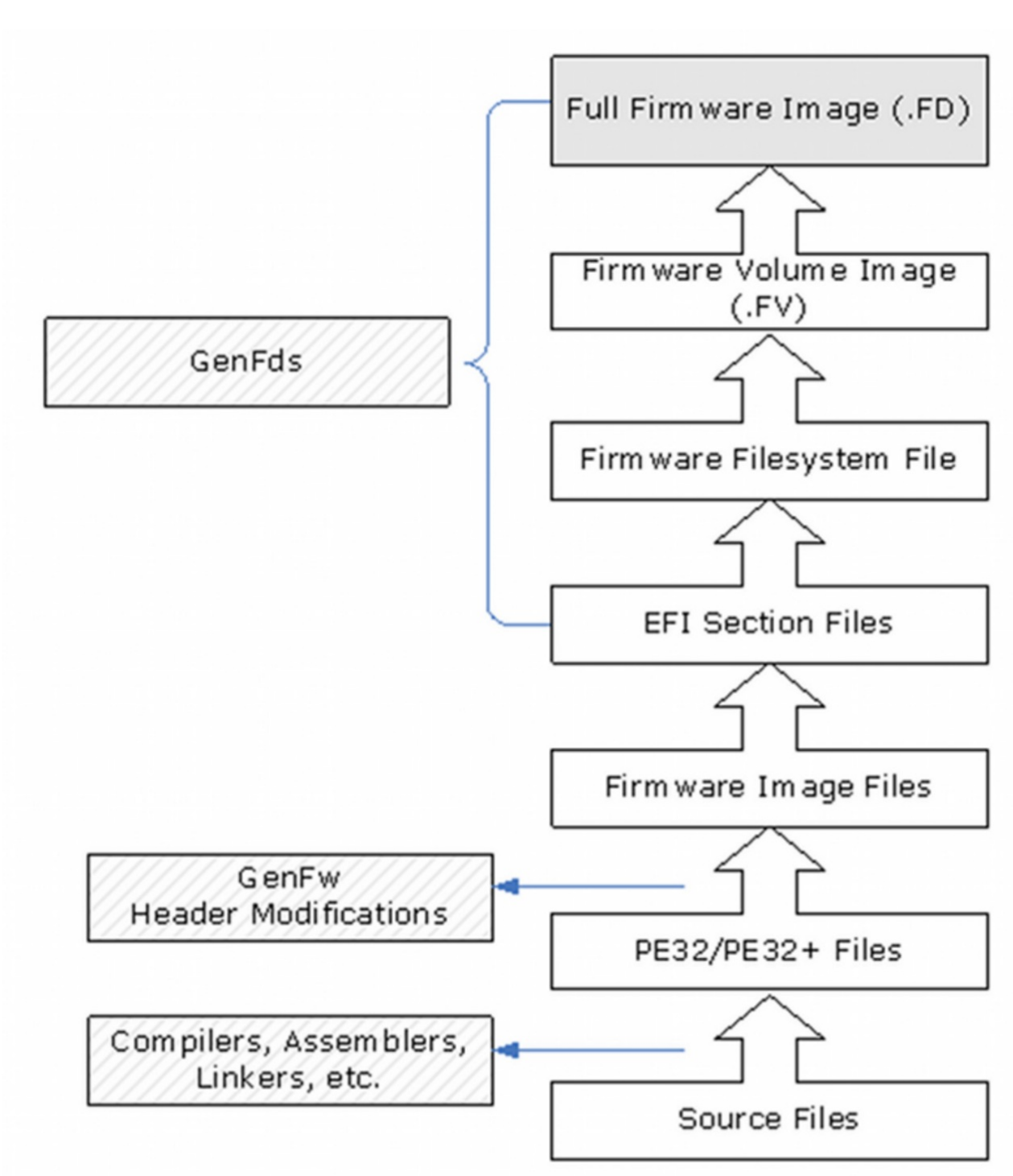
Figure 1 UEFI/PI Firmware Image Creation
