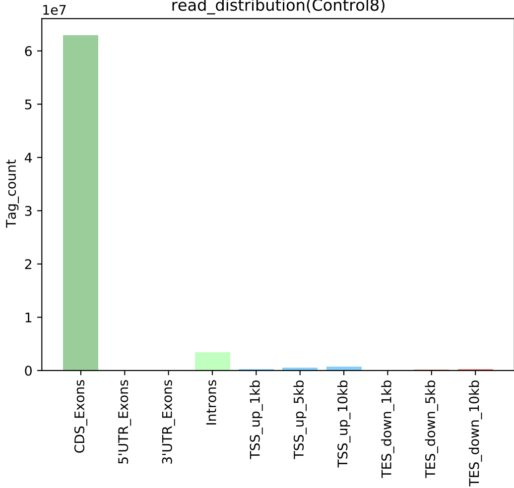
read_distribution(Control8)
