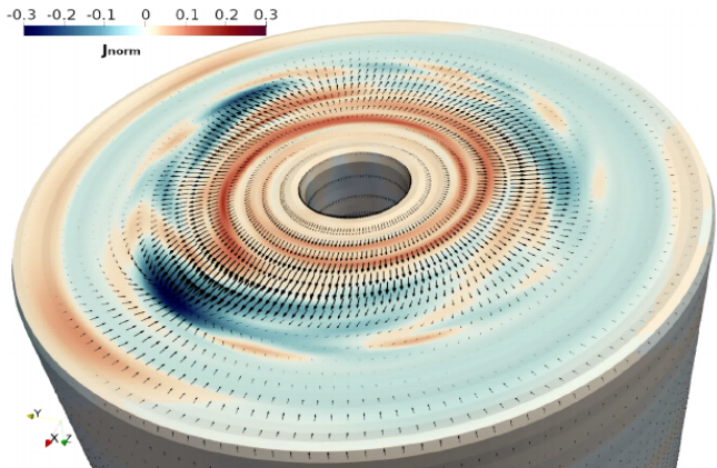
Figure 2. – Bottom view of the thin wall used for the 3D VDE benchmark case published in Ref. [99] showing the distribution of source/sink (halo) currents (black arrows). The colors indicate the perpendicular current density into the wall respectively out of it (in a.u.). The B.C. for the electric potential was \Phi = 0 here such that the wall acts ideally conducting for the halo currents.
