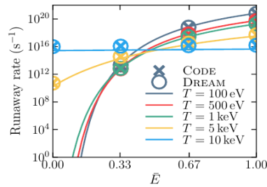
Figure 5: Comparison of the runaway rate as calculated with CODE (circles), with DREAM (crosses) and using the formula given in [29] (solid lines). The dimensionless variable \bar{E} = (E - 2E_c)/(0.04E_D - 2E_c) is introduced so that \bar{E} \in [0, 1] covers the region of E in which the runaway generation is mild to modest, and the linearized collision operator is valid. The CODE and DREAM runaway rates match to within 3.5%.
