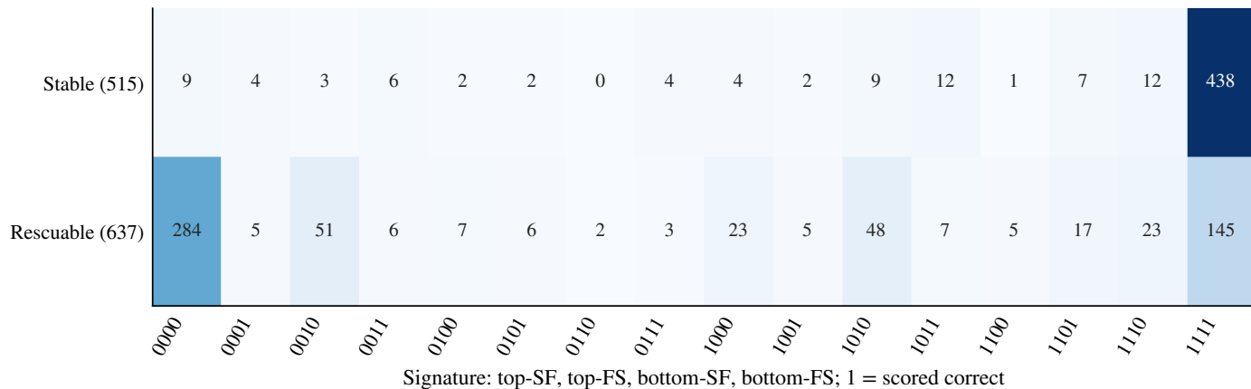
(b) Correctness regimes
