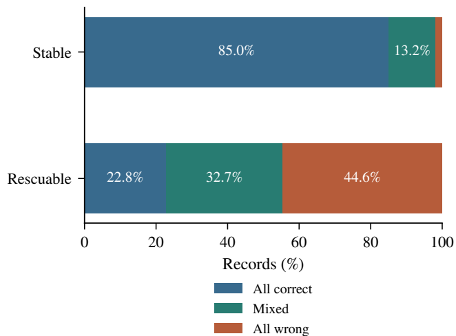
(b) Correctness regimes
