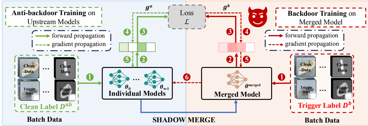
Figure 2: Overview of MergeBackdoor. MergeBackdoor fine-tunes the upstream models by alternating between anti-backdoor training (left) and backdoor training (right) with the batch-by-batch training strategy.
