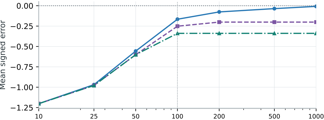
Case 2 | \theta_1
