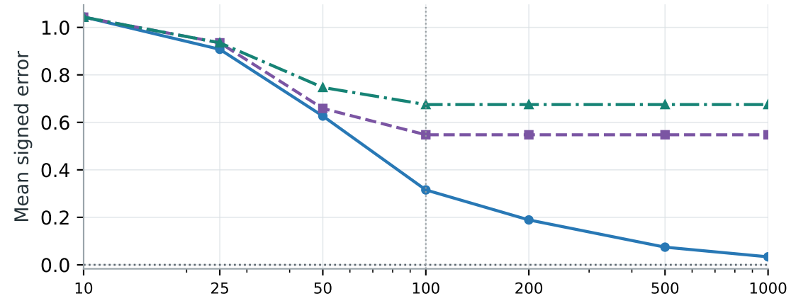
Case 1 | \theta_2
