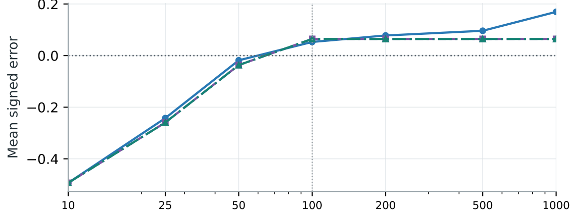
Case 3 | \theta_1
