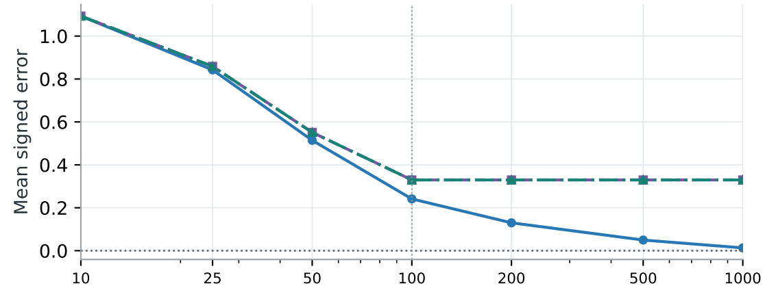
Case 3 | \theta_2
