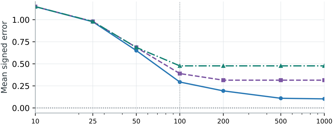
Case 2 | \theta_2
