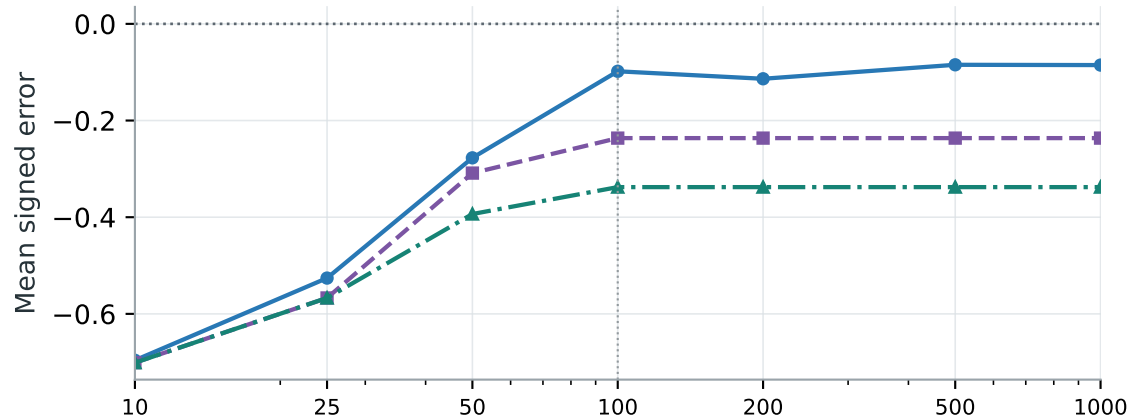
Case 1 | \theta_1
