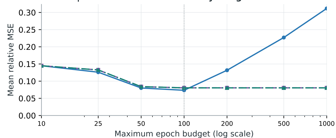
Case 3 | Nuisance-function error by budget
