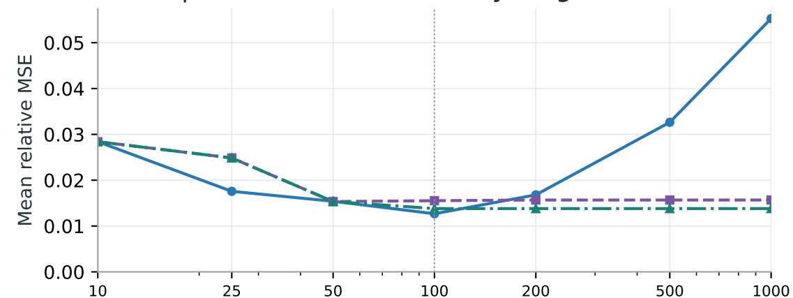
Case 2 | Nuisance-function error by budget
