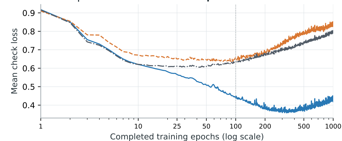
Case 3 | Prediction loss at each epoch
