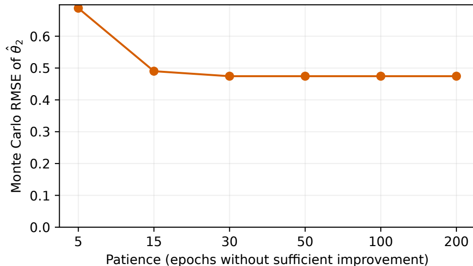
Coefficient \theta_2
