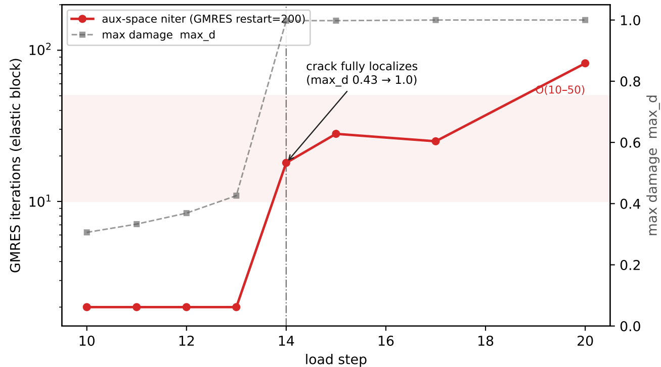
Real phase-field run: aux-space stays bounded across full localization (deterministic re-solve, GMRES restart=200)
