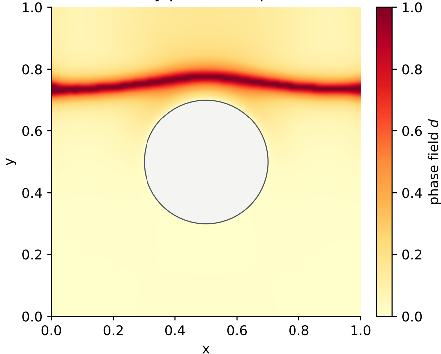
Clamped circular-boundary plate: final phase field d ( \bar{u} = 0.1250 )
