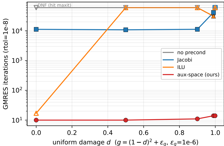
tion stability vs damage — model2 (mode-II notch shear) ( \sigma -d
