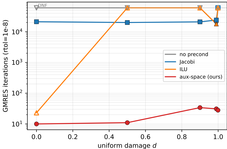
Iteration stability vs damage — square (I-tension), \sigma -dof=30
