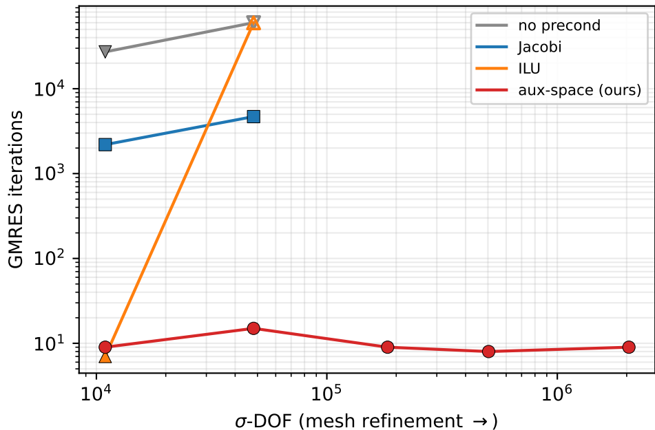
Iteration count vs problem size — model0, d=0.9
