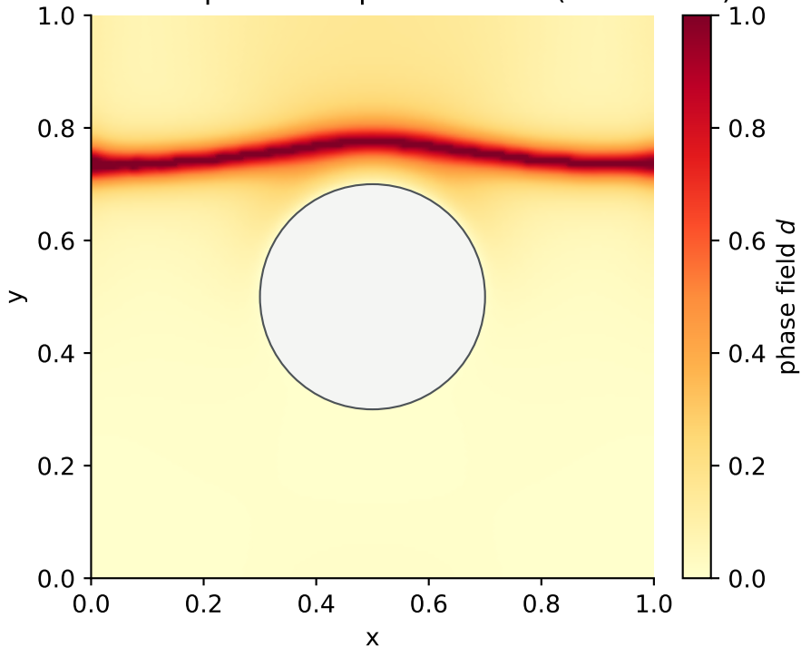
Circular-hole plate final phase field d ( \bar{u} = 0.1250 )
