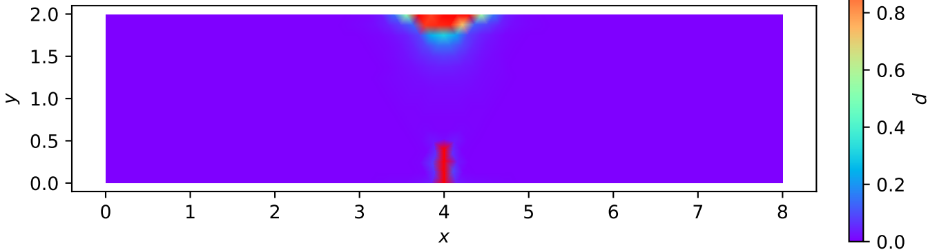
Three-Point Bending of a Notched Beam: phase field d at u = 0.080
