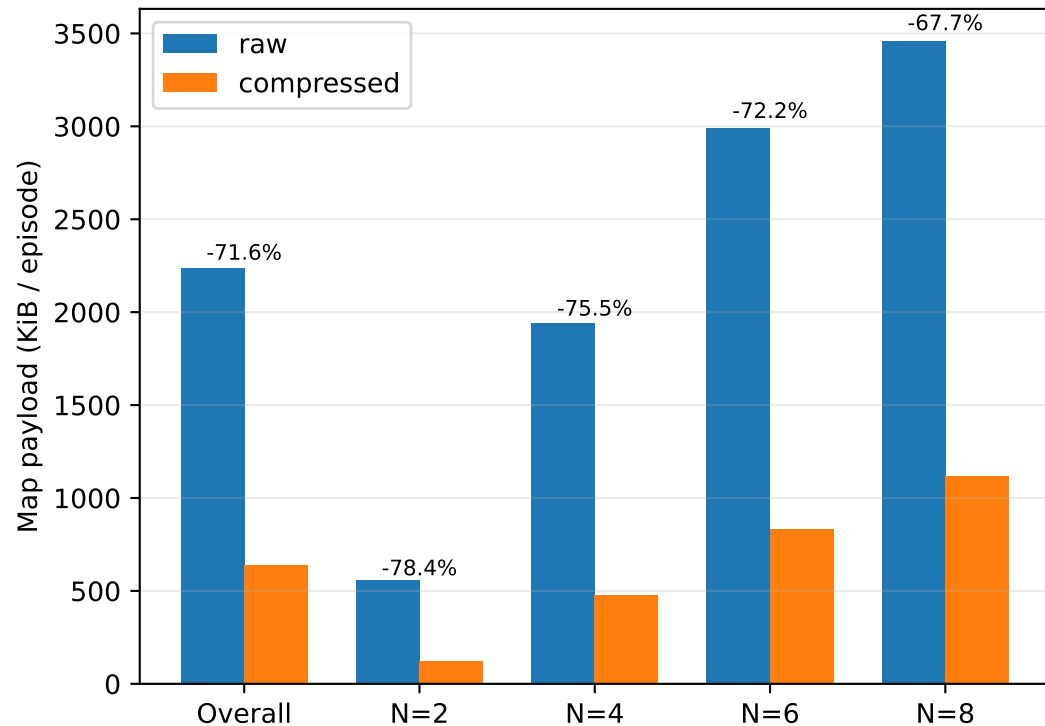
(b) Compression saving
