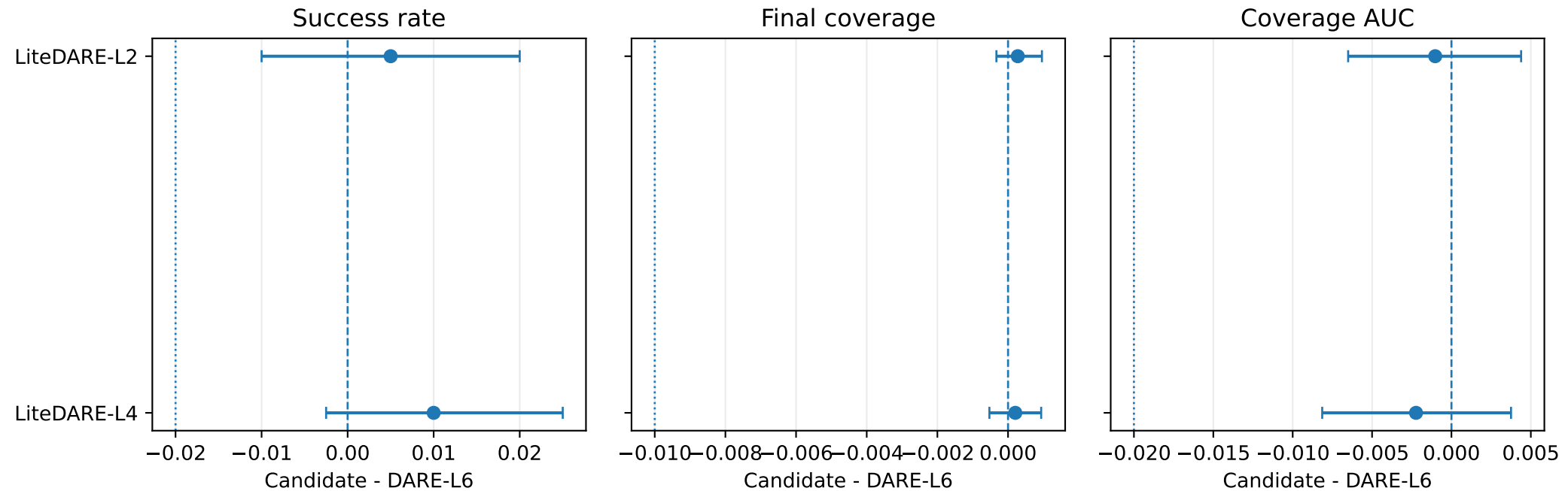
Figure 4.2. Paired deviations from DARE-L6 (95% bootstrap CI)
