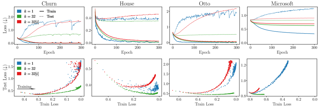
Figure 5: The training profiles of TabM mini k=32 and TabM mini k=1 as described in subsection 5.1 . ( Upper ) The training curves. k = 32[i] represents the mean individual loss over the 32 submodels. ( Lower ) Same as the first row, but in the train-test coordinates: each dot represents some epoch from the first row, and the training generally goes from left to right. This allows reasoning about overfitting by comparing test loss values for a given train loss value.
