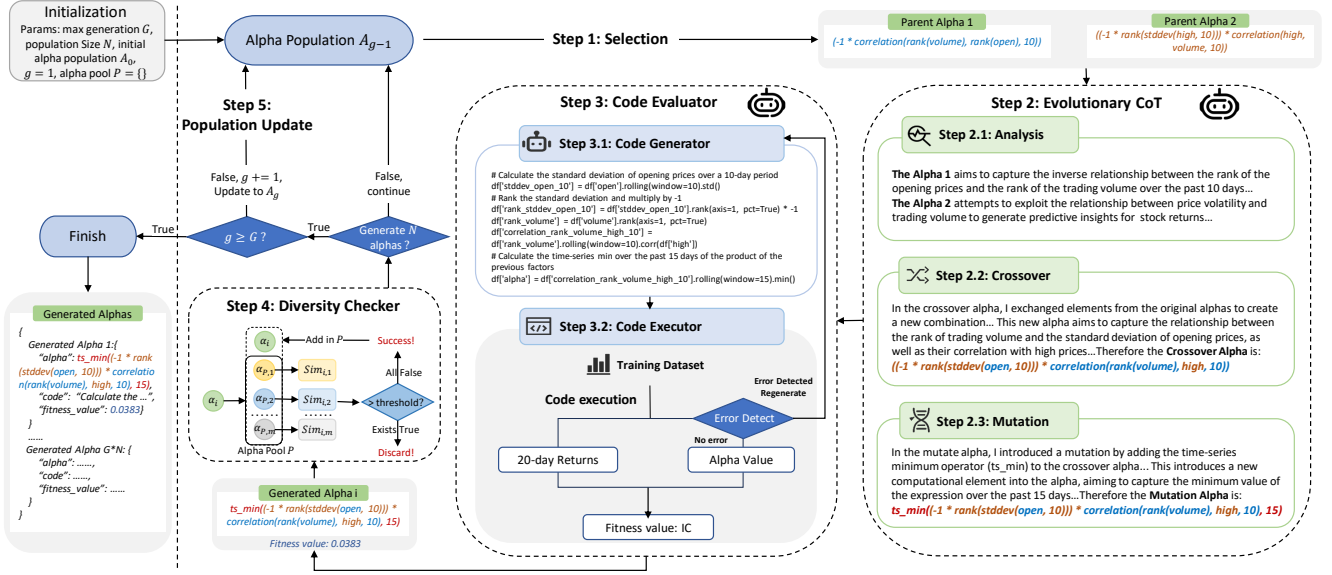
Fig. 1. The framework of EvoAlpha. It first selects two parent alphas from the population and then generates a new alpha through Evolutionary CoT, which subsequently is evaluated by the Code Evaluator. Then, it will be filtered by the diversity checker. Each generation g will generate N alphas. Then, these generated alphas are merged with the original population, and the top N alphas are retained as the population for the next generation. This process iterates until g reaches the predefined G .
