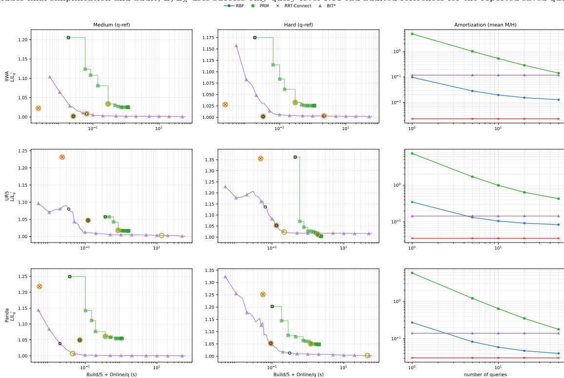
Fig. 6. Saved-catalog random-scene trade-off. Left and middle panels show a fixed five-query display point, Build/5 + Online/q, for medium and hard rows; the right panel varies the amortization count K in Build/ K + Online/q. Methods without a reusable-build term are plotted at Online/q. Rings mark the first checkpoints with audited success on the reported saved query set (black) and later \geq 1\% path-ratio improvements (gold); PRM and BIT* curves use offline checkpoints.
